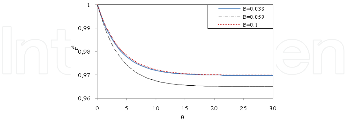
Fig. 6. Low temperature versus heat transfer time for B=0.1,0.059,0.038 .
