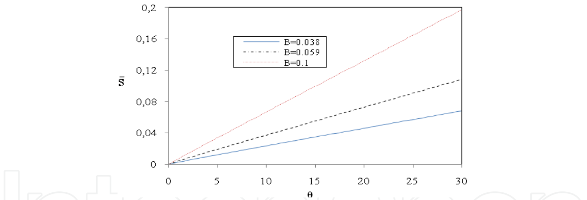
Fig. 12. Transient behavior of entropy generated during the time ( \tau_H=1.3 and \tau_{st}=1.6 ).
