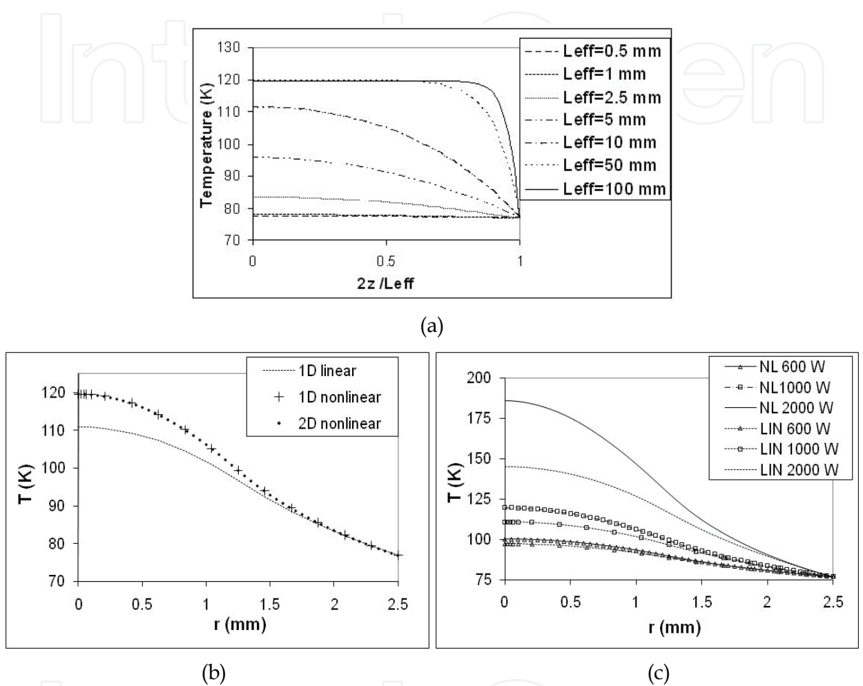
Fig. 2. Temperature in a rod: a) axial distribution for heat density of 410 W/cm 3 , b) radial distribution for heat density of 410 W/cm 3 , comparing rod with finite and infinite length and with the linear solution, and c) radial distribution for heat density of 245, 410 and 815 W/cm 3 , comparing the nonlinear with linear solutions
