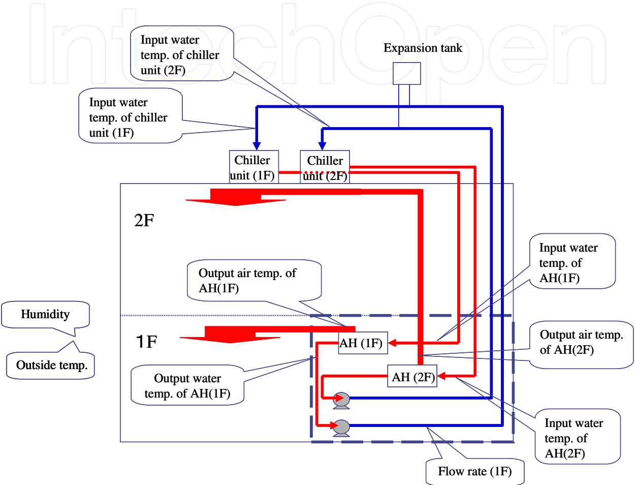
Fig. 15. Schematic diagram of the air conditioning system. (AH: Air Handling Unit)
