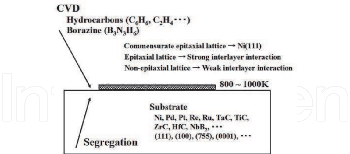
Fig. 1. A schematic diagram of growing processes of graphene and h-BN films by CVD or surface segregation techniques on solid surfaces.
