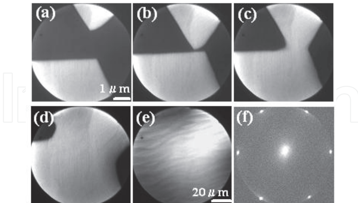
Fig. 6. Typical snapshots of LEEM images obtained as the temperature was decreased from 1200 K to 1125 K (images (a) to (d)). The observed area was 6 \mu\text{m} field-of-view. Letter in each image indicates the time-lapse order. Two graphene domains were united to form one graphene sheet. Image (e) is a typical LEEM image of 100 \mu\text{m} field-of-view. The surface was entirely covered with monolayer graphene. LEEM images were obtained at the primary electron energy of 3.5 eV. Image (f) is a typical \mu\text{LEED} pattern observed in the graphene-covered surface. The orientation of the graphene was slightly altered because the sheet is curved.
