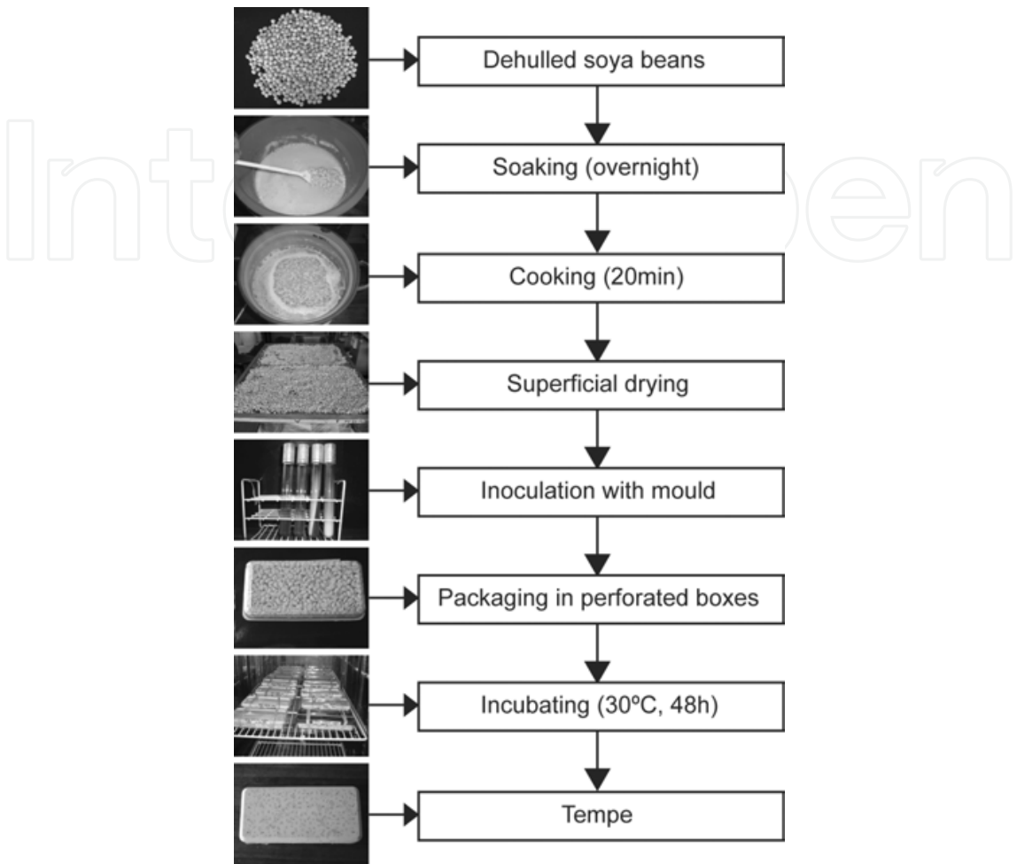
Fig. 3. Production process of soya bean tempe.
