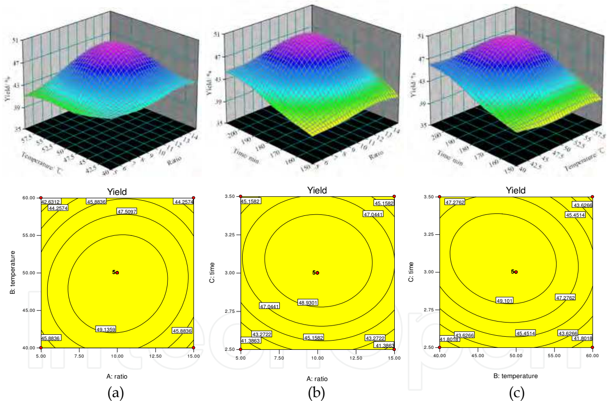
Fig. 1. Two and three dimensional contour plots for the maximum yield of nanocellulose. RSM plots were generated with the data shown in Table 2. (a) Yield of nanocellulose (%) as a function of ratio of NKC-9 to MCC and temperature. (b) Yield of nanocellulose (%) as a function of ratio of NKC-9 to MCC and time. (c) Yield of nanocellulose (%) as a function of temperature and time.
