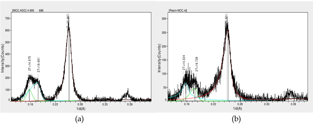
Fig. 4. XRD patterns of (a) NCC and (b) MCC.
