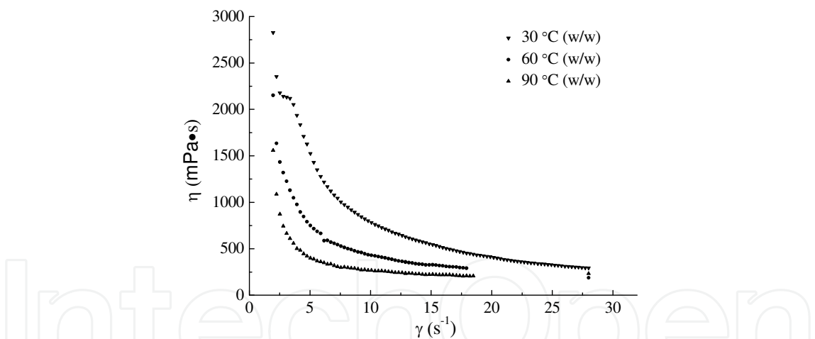
Fig. 9. Variation of the viscosity with a function of shear rate of NCC suspension at various temperatures.
