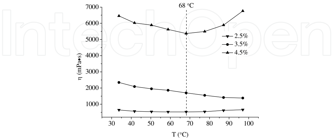
Fig. 8. Variation of the viscosity with a function of the temperature of NCC suspensions at various concentrations.
