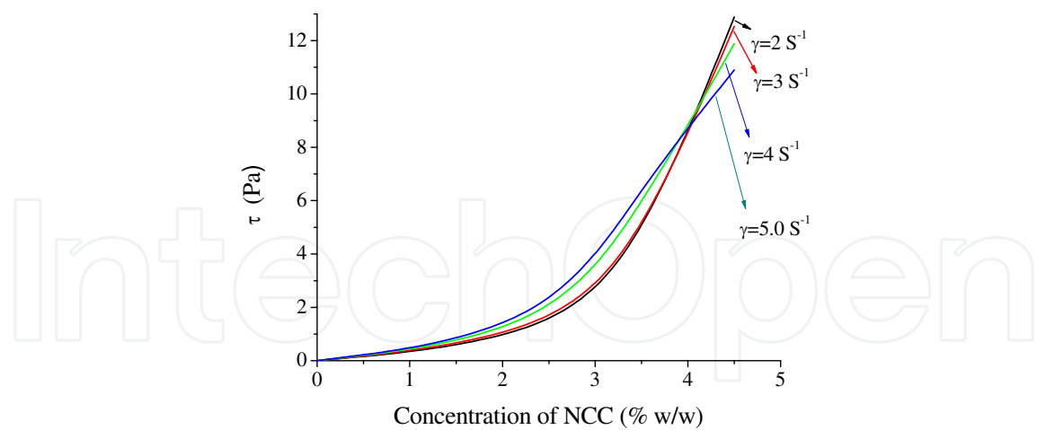
Fig. 6. Variation of the stress with the function of concentration of NCC at various shear rates.
