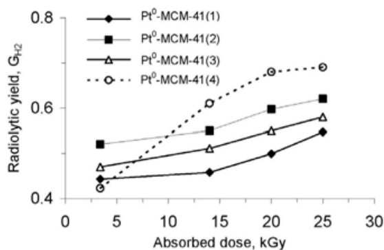
Fig. 6. Plots of radiolytic yield vs. absorbed dose for: a) Pt 0 -MCM-41 impregnated samples for 1) short temps 2) long temps, 3) before irradiation, 4) after irradiation.
