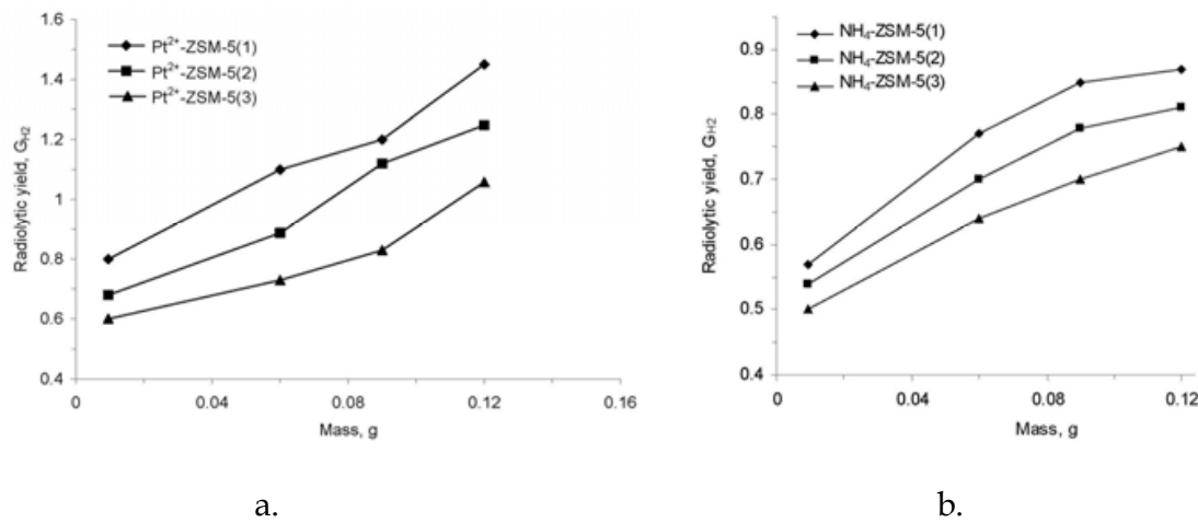
Fig. 1. Plots of radiolytic yield vs catalyst mass for a) Pt 2+ -ZSM -5 and b) NH 4 -ZSM-5 with different SiO 2 / Al 2 O 3 ratios SiO 2 / Al 2 O 3 = 140, (2) SiO 2 / Al 2 O 3 = 80, (3) SiO 2 / Al 2 O 3 = 15.
