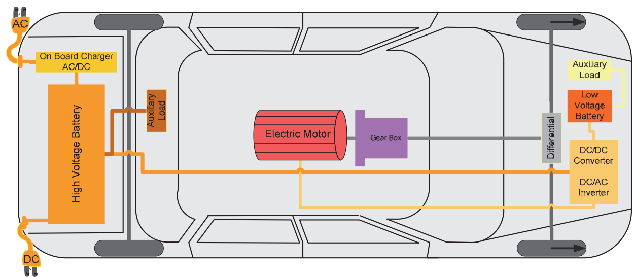
Fig. 3. Electric Vehicle Model
