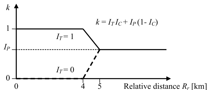
Fig. 7. Image of uncertainty coefficient with uncertain information.
