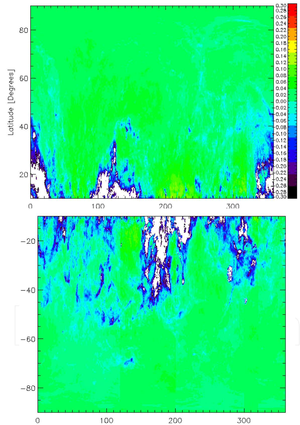
Fig. 12. Map in galactic coordinates of \delta E(B - V) from the comparison of AL07 model with SFD98 for the whole Galaxy, using a grip spacing of 0.25^\circ in l and b (Adapted from AL07, figure 3).
