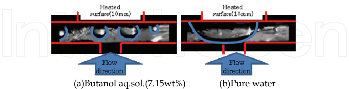
Fig. 23. Behaviour of boiling bubbles (T-junction mini tube made of polymer material).
