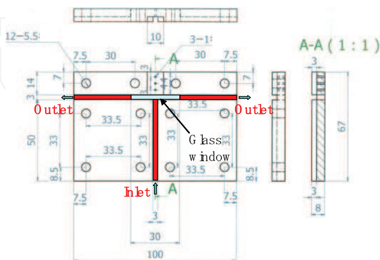
Fig. 22. Test section (T-junction mini tube made of polymer material).
