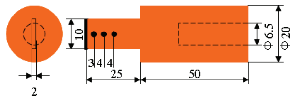
Fig. 19. Copper block used for heating.
