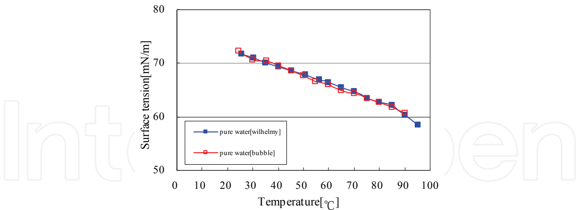
Fig. 4. Pure water data obtained using the maximum bubble pressure method and Wilhelmy’s method.
