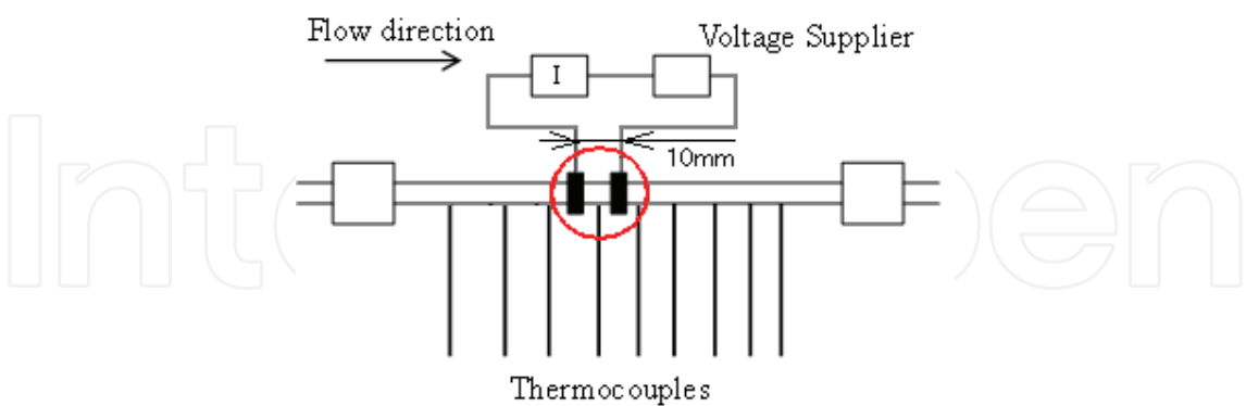
Fig. 12. Test section with the short heating length of D_{in} = 1\text{ mm} .
