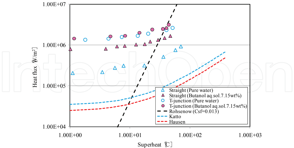
Fig. 24. Boiling curves (T-junction and straight mini tube made of polymer material).
