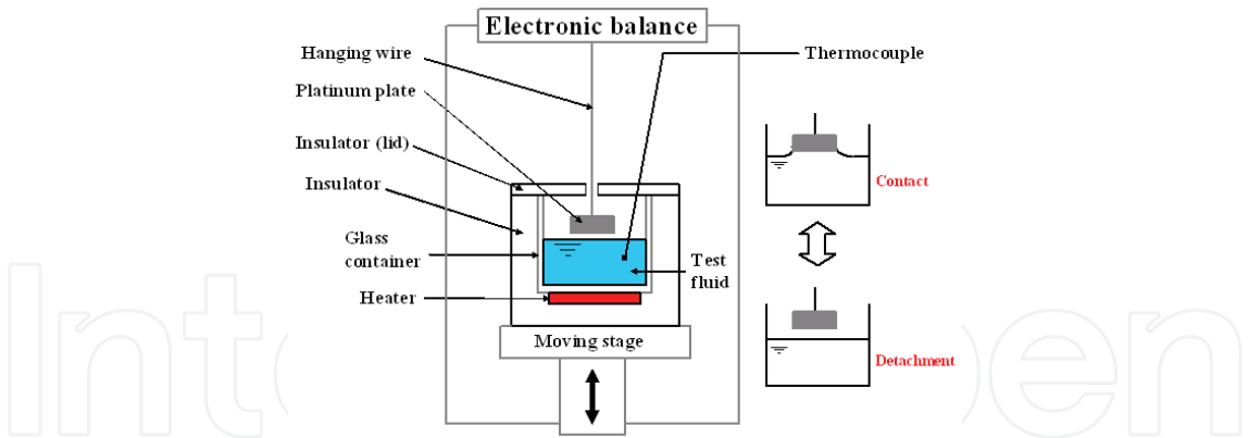
Fig. 3. Experimental apparatus for Wilhelmy’s method.
