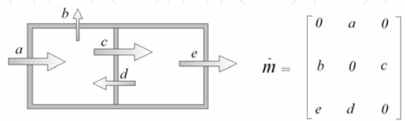
Fig. 3. Interzonal airflow rates matrix
