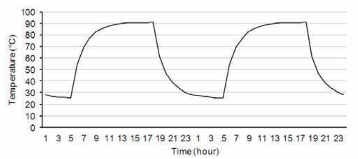
Fig. 10. Evolution of air temperature at the output of the solar collector with forced convection (1m 3 .h -1 ).
