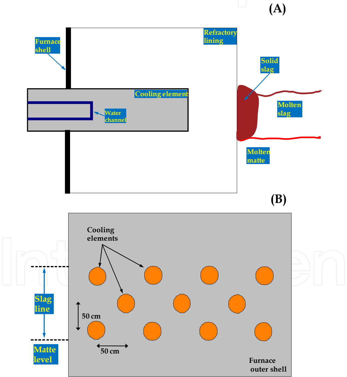
Fig. 10. Schematics of the “finger” cooler cooling device: (A) as it is embedded in the refractory lining. (B) Distribution of the cooling elements alongside the furnace slag line.
