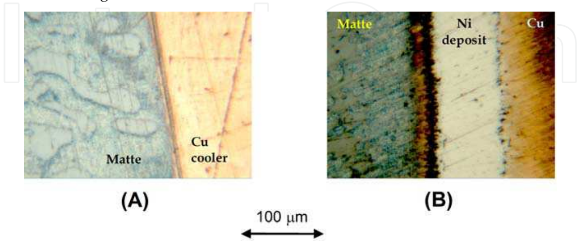
Fig. 8. Metallographs of different cooling elements after immersion in matte. (A) copper cooler, (B) Ni-plated copper cooler.
