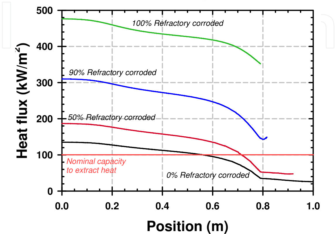
Fig. 14. Heat flux through the copper fingers and the refractory layer (computed).
