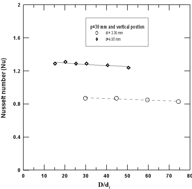
Fig. 15. Nusselt number versus D/d_i ratio.
