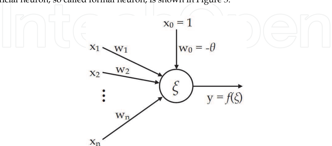
Fig. 3. Formal neuron
