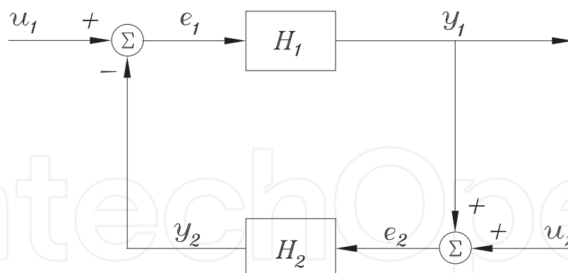
Fig. 3. Feedback connection
