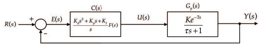
Fig. 6. PID controller based on Smith predictor characteristics
