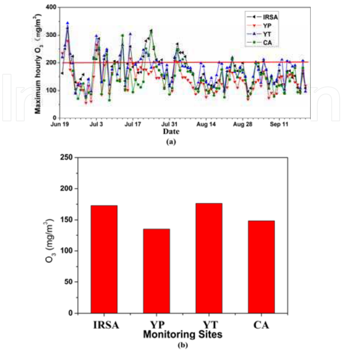
Fig. 12. Maximum hourly ozone concentrations on a daily basis and statistical average of the maximum hourly ozone during the whole campaign
