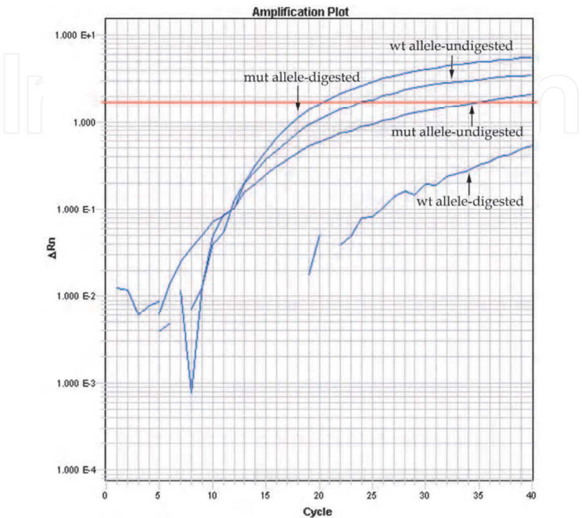
Fig. 4. TspRI digestion increases the sensitivity of the BRAFV600E allele-specific real-time PCR. The amplification plot shows that the complete elimination of the BRAF wild-type template by TspRI digestion improves the sensitivity of mutated allele-specific PCR, anticipating its detection of about 14 cycles compared to undigested samples. The red line represents the threshold line. wt: wild-type. mut: mutated.
