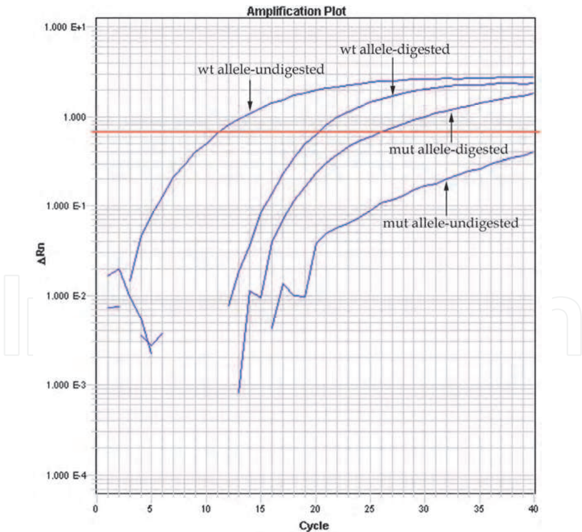
Fig. 3. TspRI digestion increases the specificity of BRAFV600E allele-specific real-time PCR.
