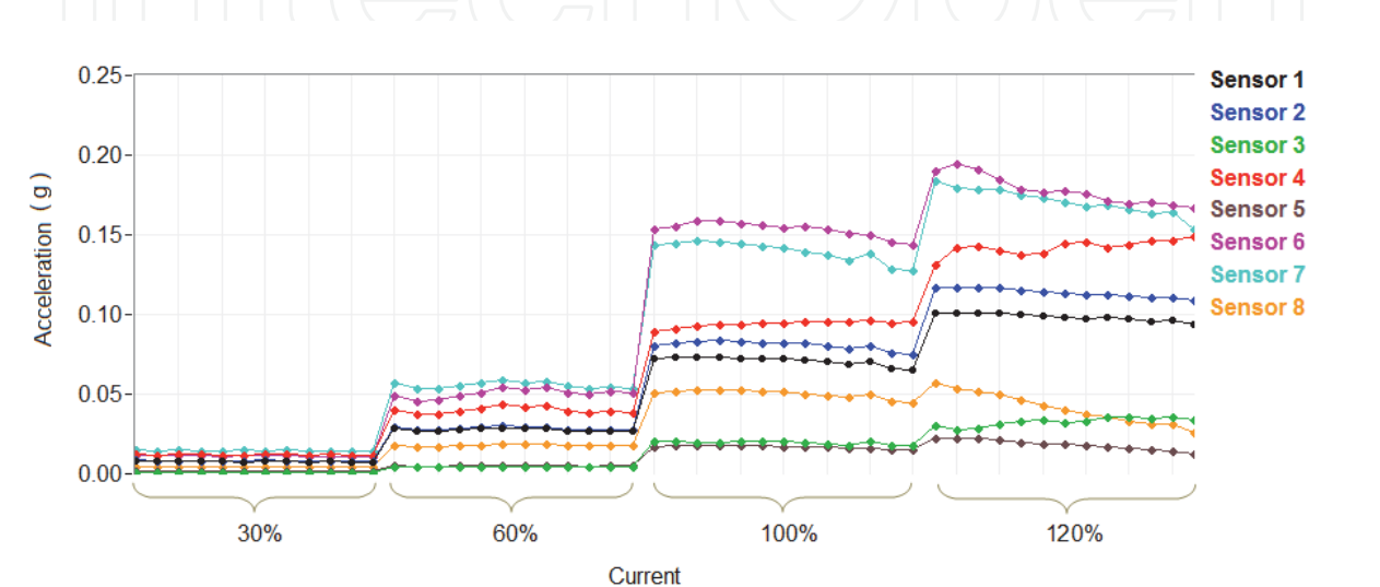
Fig. 7. Vibration signals when excited with current at 120 Hz. in all sensors.
