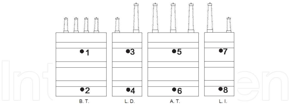
Fig. 5. Location of the sensors in the transformer. Two in the low voltage side (B.T.), the following in the right side (L.D), two in high voltage side (A.T) and the last in the left side (L.I).
