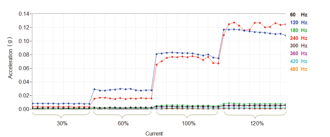
Fig. 8. Vibration signals when excited with current at sensor 2 in all frequencies.
