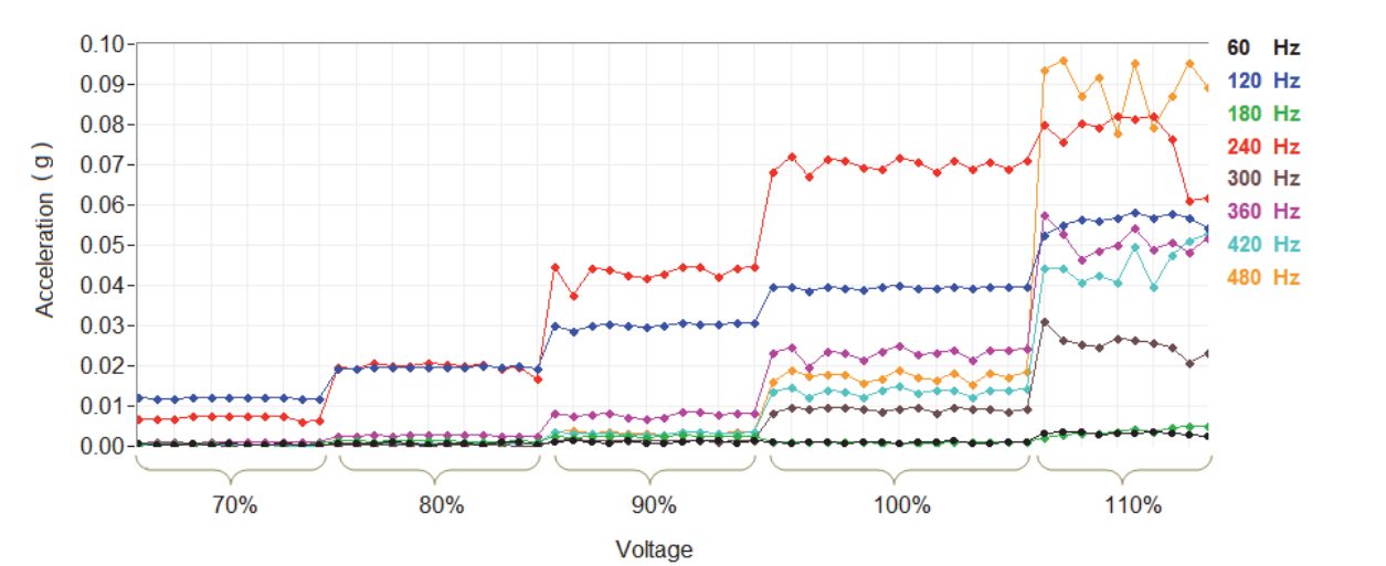
Fig. 10. Vibration signals when excited with voltage at sensor 2 in all frequencies.
