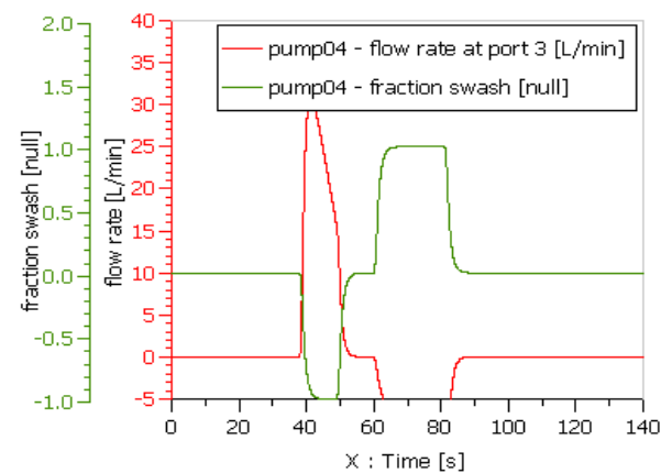
(g) Evolution of oil flow inside the accumulators depending on control signal of the hydrostatic unit capacity
