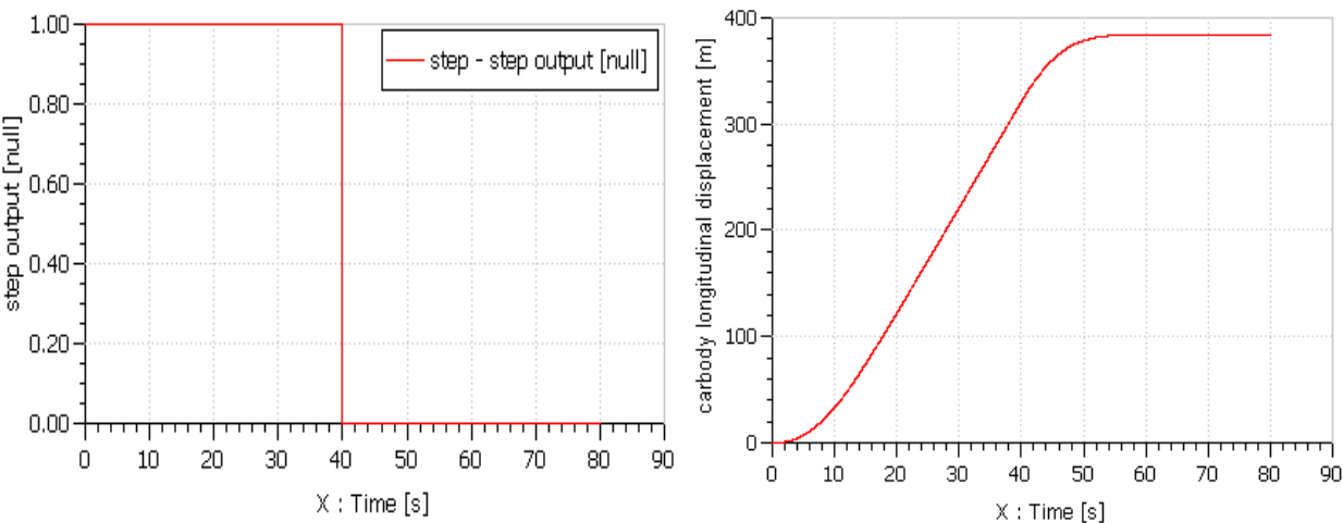
(a) Variation over time of control signal of heat (b) Evolution over time of displacement of vehicles
