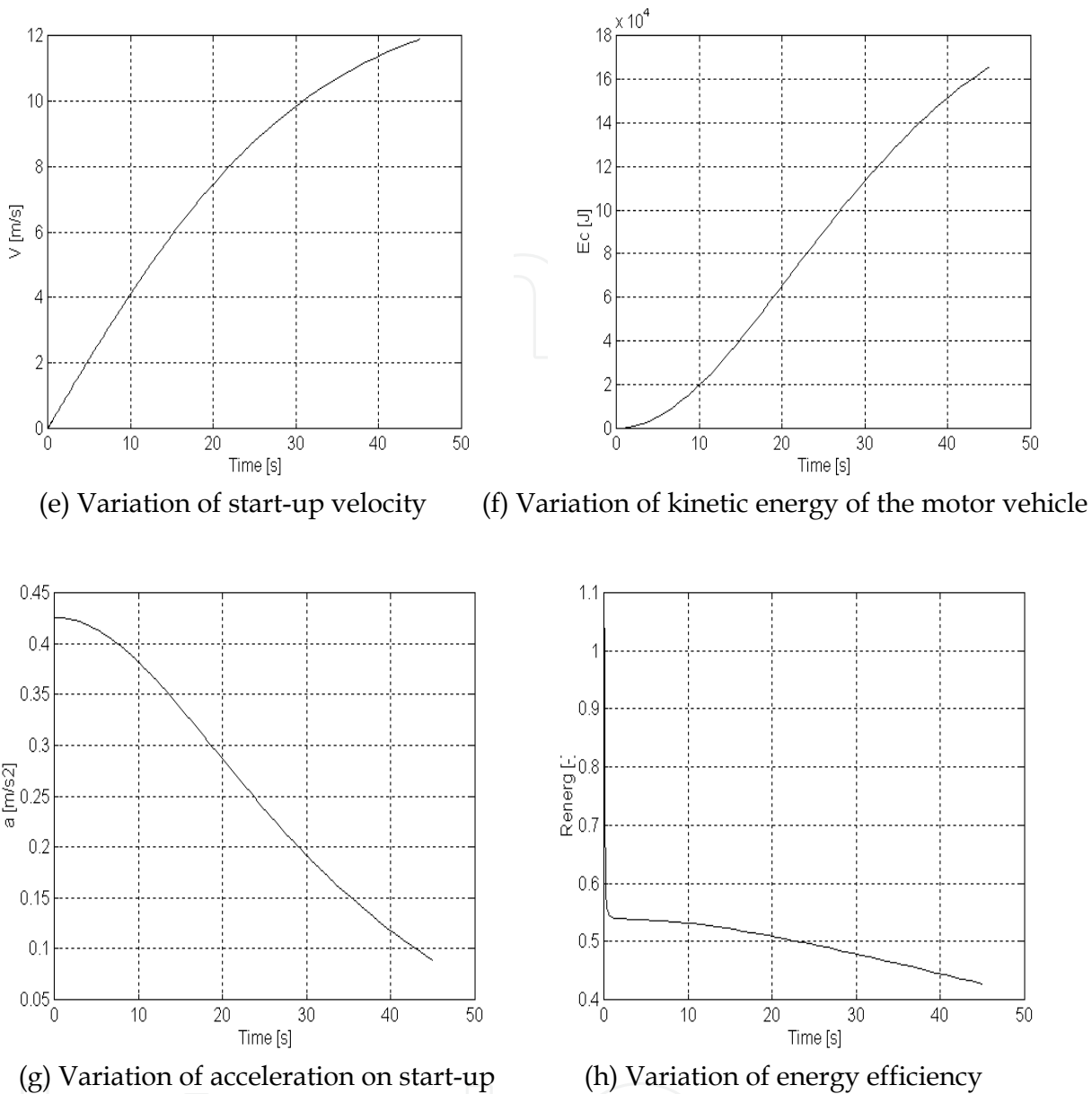
Fig. 12. Variation of the main parameters of hydraulic starting process of a motor vehicle. In the Figures 12, there are presented some theoretical results of interest regarding the dynamic behavior of the motor vehicle at its hydraulic start-up. Thus, the variation of oil and gas volumes are shown in Figure 12(a), where it can see that the oil volume is in decreasing and the gas volume is in continuous increasing. The pressure in the accumulators is in continuous decreasing, as see in Figure 12(b). The variation of start-up stroke is shown in Figure 12(c). The Figure 12(d) highlights the existing of a maximum value of the power at e hydraulic motor (HM). The variation of start-up velocity is done in Figure 12(e) and this corresponds with the variation of kinetic energy of the motor vehicle, which is shown in Figure 12(f). The variation of acceleration on start-up of the vehicle is presented in Figure 12(g). The variation of energy efficiency of hydraulic propulsion is shown in Figure 12(h) and is around of 60%. The pressure variation in accumulators is done by the next relation (4):
