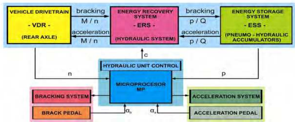
Fig. 4. General systemic model of the command and control system.
