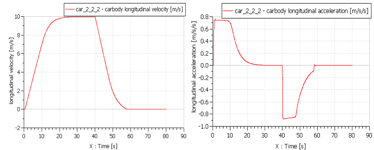
(c) Evolution of running velocity of motor vehicle (d) Evolution over time of acceleration of vehicles
