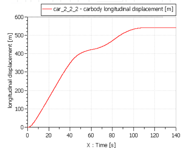
(a) Evolution over time of displacement of motor vehicle
