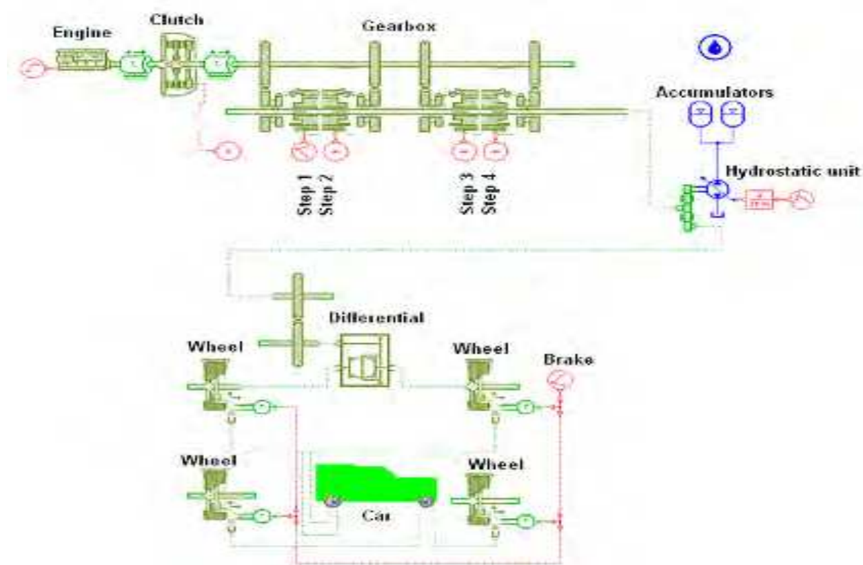
Fig. 20. The simulation network of the dynamic behavior of the motor vehicle with thermo-hydraulic propulsion system.
