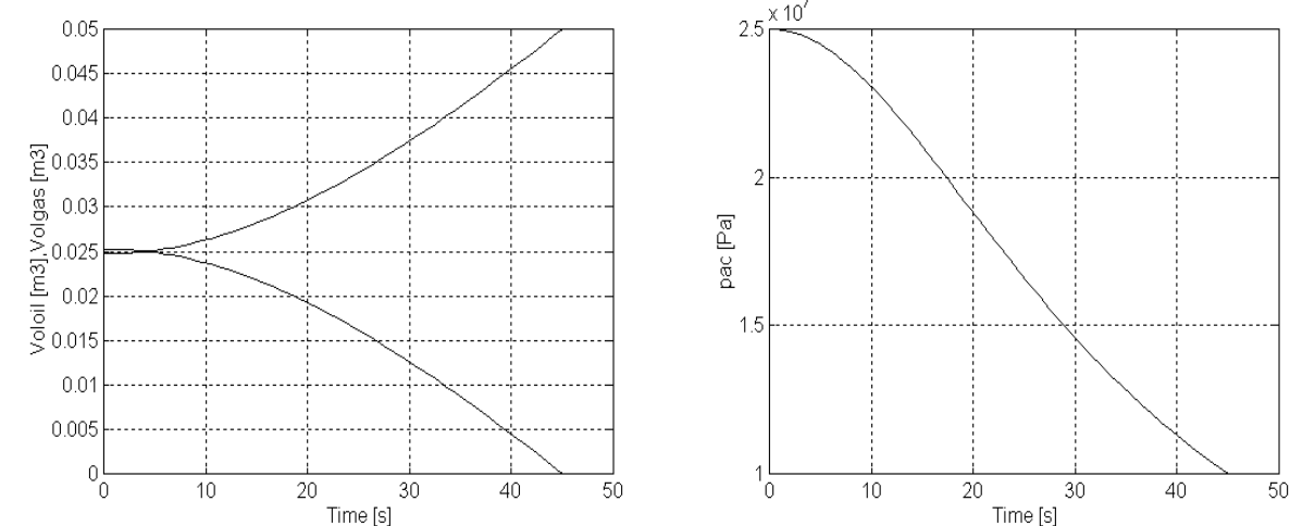
(a) Variation of oil and gas volumes (b) Variation of pressure inside the accumulators
