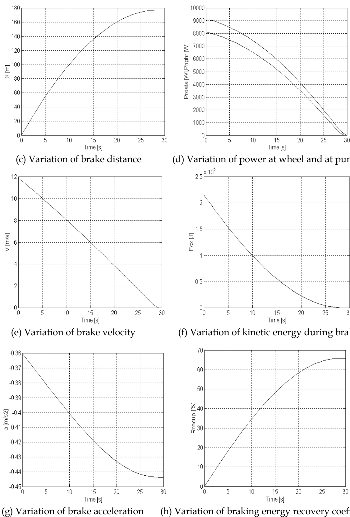
Fig. 15. The variation of the main dynamic parameters of the braking process with energy recovery.
