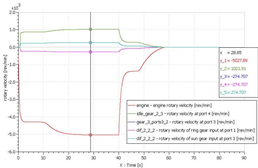
(g) Variation of rotational speed at the heat engine shaft, gearbox and differential
