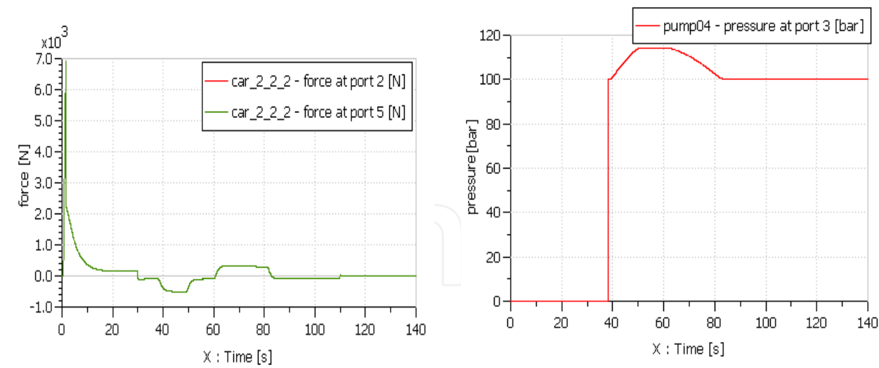
(e) Variation of force at the drive wheel (f) Evolution of pressure inside of accumulators
