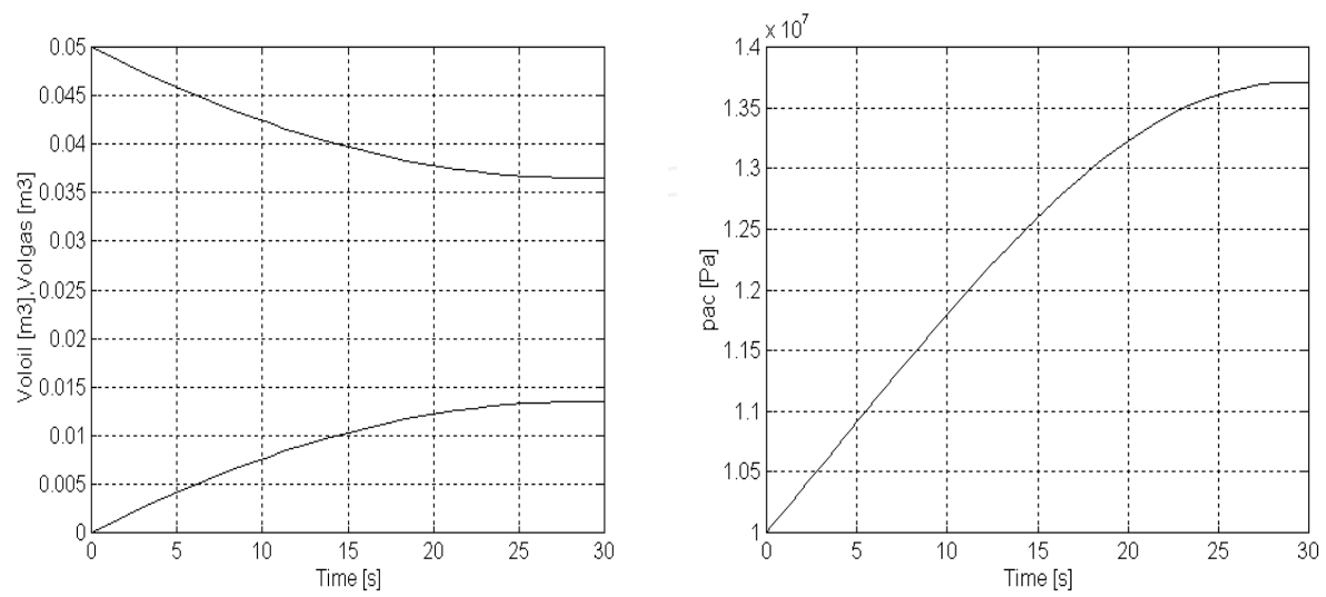
(a) Variation of volumes of oil and azotes inside the accumulators
