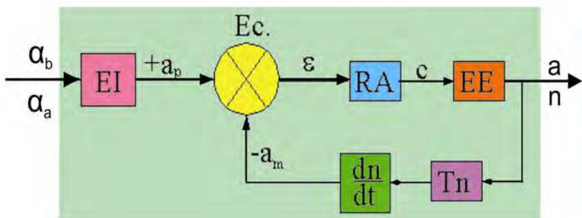
Fig. 2. Automatic adjustment schematic diagram of the hybrid propulsion system of motor vehicles.
