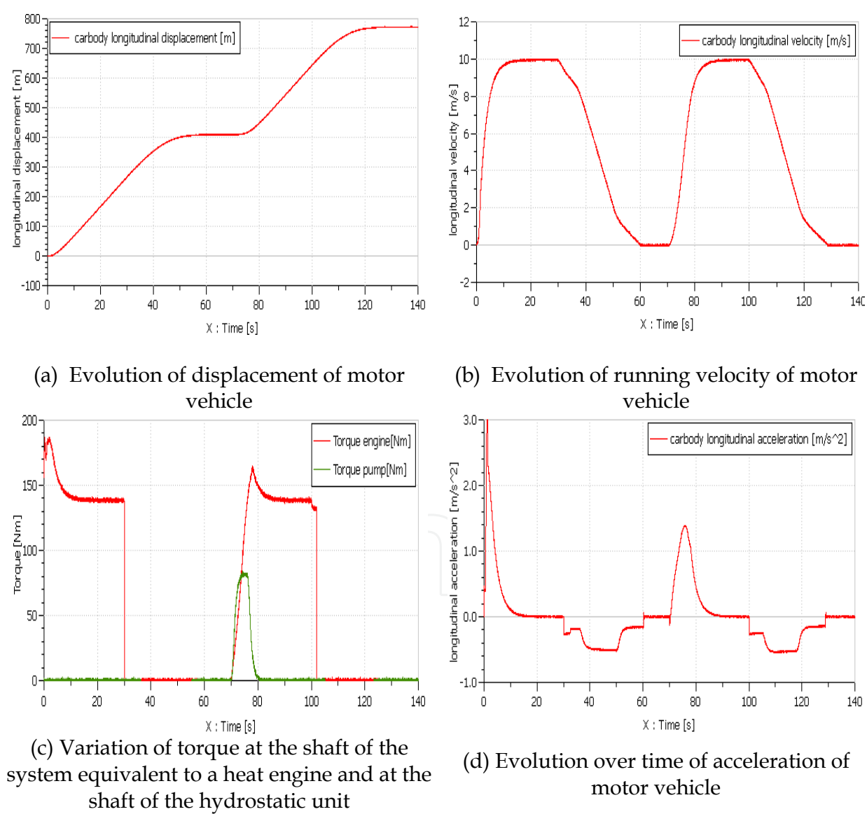
Fig. 29. Data obtained from experiments of real-time simulation for testing of energy recovery system.
