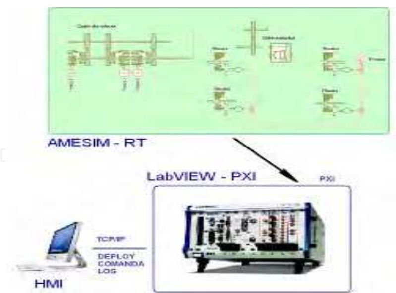
Fig. 26. Co-simulation subsystem.
