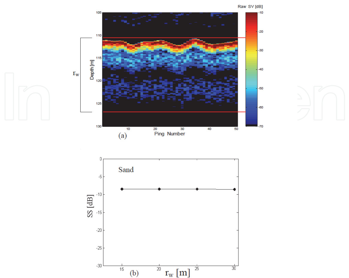
Fig. 4.3. The echogram in raw SV scale (a) and the relation of measured SS on r_w values (b). In decibel scale SA = 10 \log S_A . From Eq. (4.1) we have
