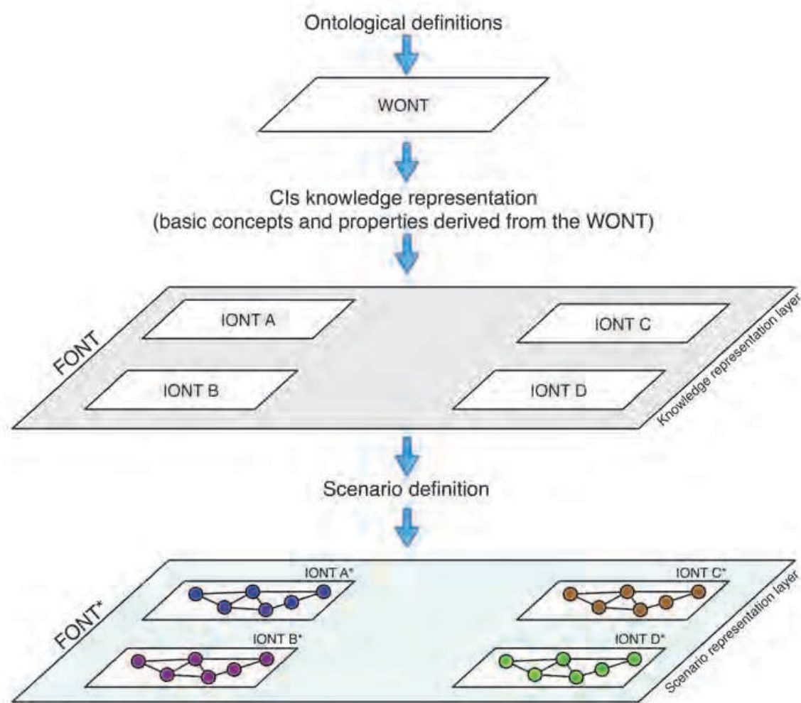
Fig. 4. KBS architecture.
