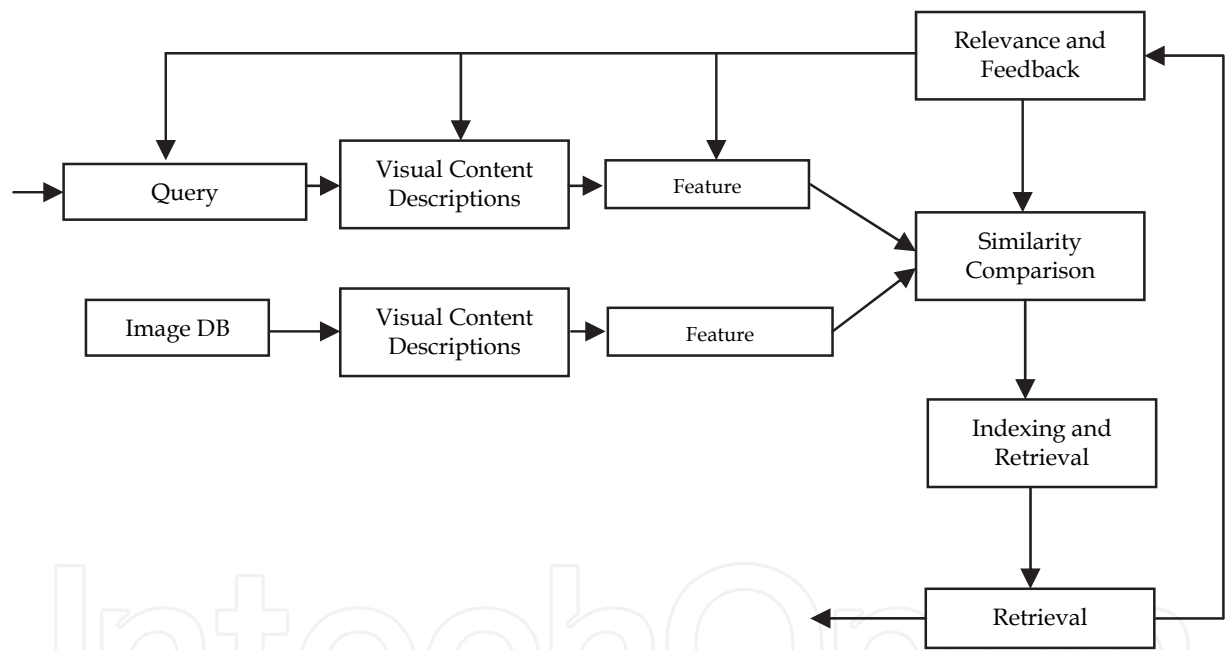
Fig. 2. Diagram of content based image retrieval system
