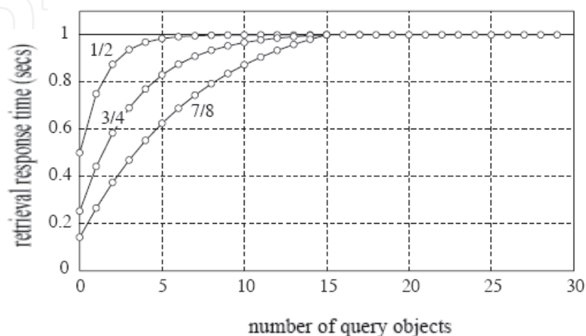
Fig. 4. Number of query objects Vs response time
