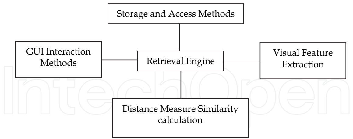
Fig. 1. Principal components of a CBIR system
