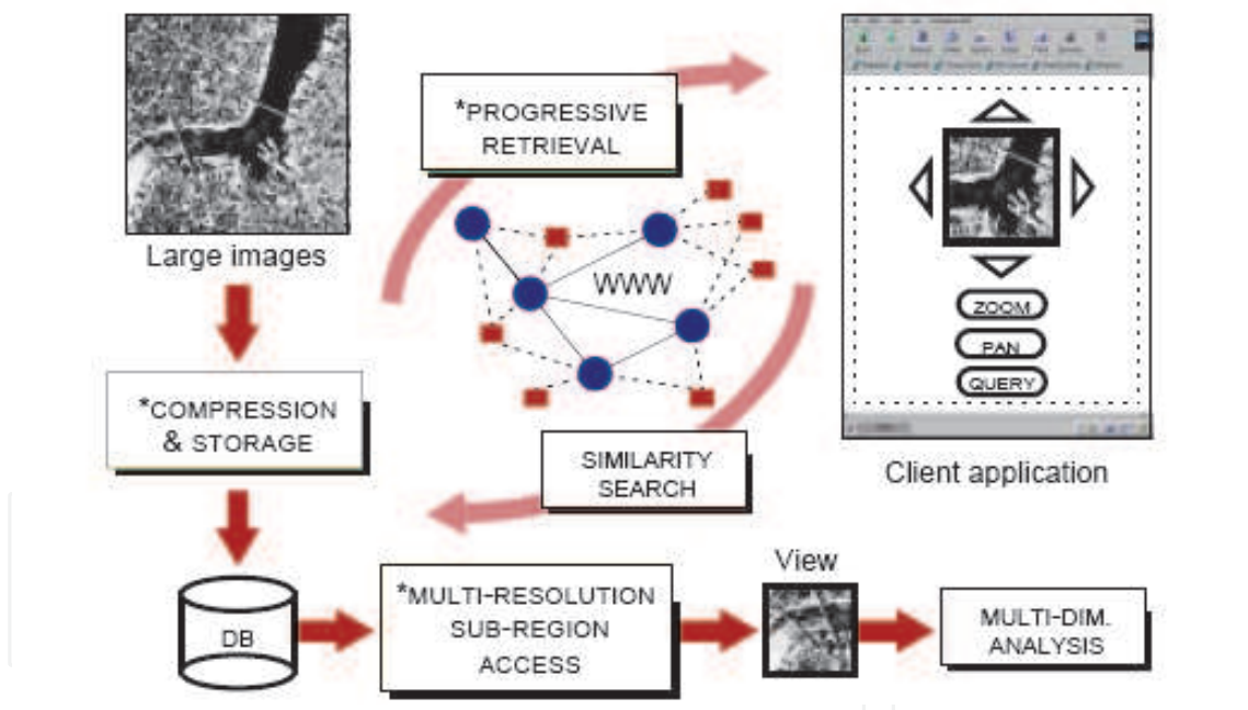
Fig. 3. Large Image Storage and Retrieval Environment
