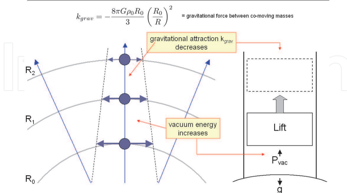
Fig. 1. Schematic illustration of the physical action of a constant vacuum energy density and of inter-material cosmic gravitational fields requiring work to be done, if co-moving matter is transferred to larger cosmic scales S = R .
