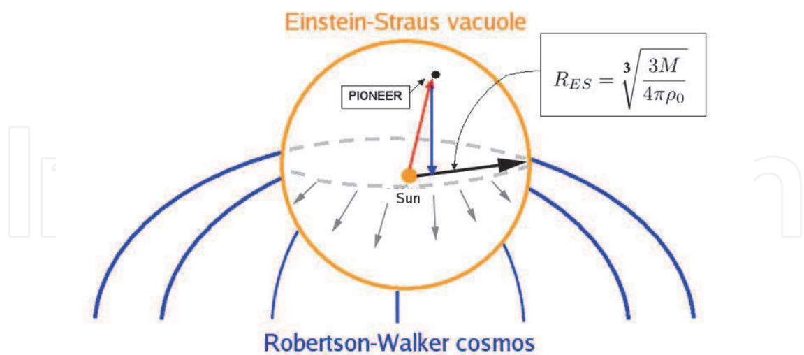
Fig. 2. Visualization of the Einstein-Straus globule surrounding a mass M within the expanding Robertson-Walker universe.
