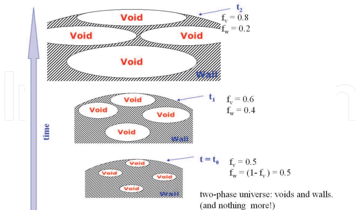
Fig. 4. Illustration of the non-homologous expansion of a two phase universe with void and wall regions having different matter densities.
