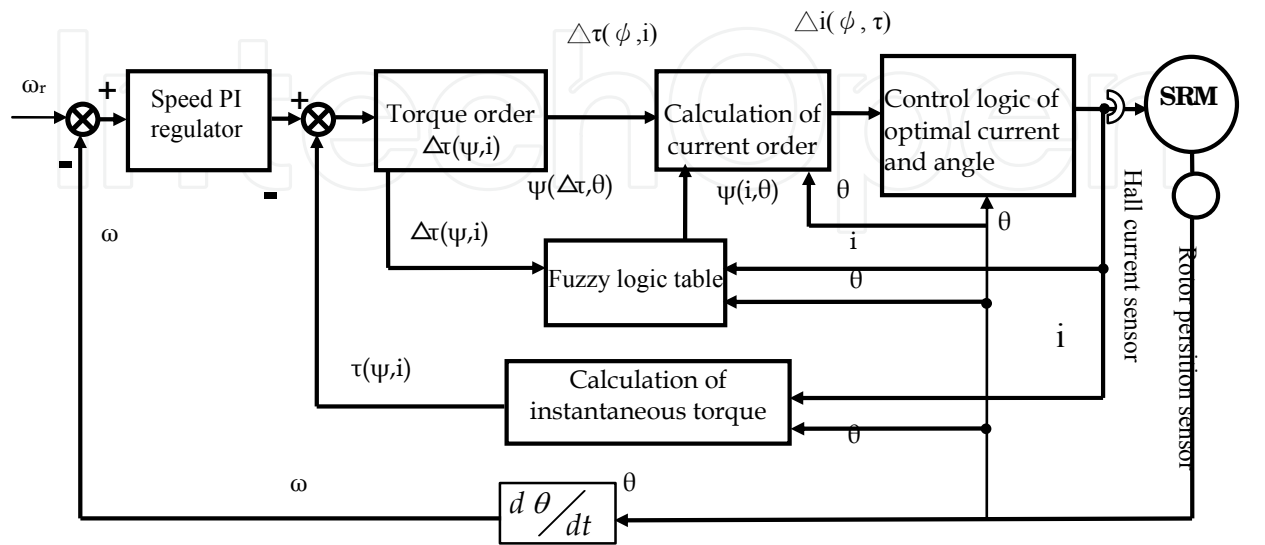
Fig. 14. Principal frame of SRM fuzzy logic adaptive direct torque control system
