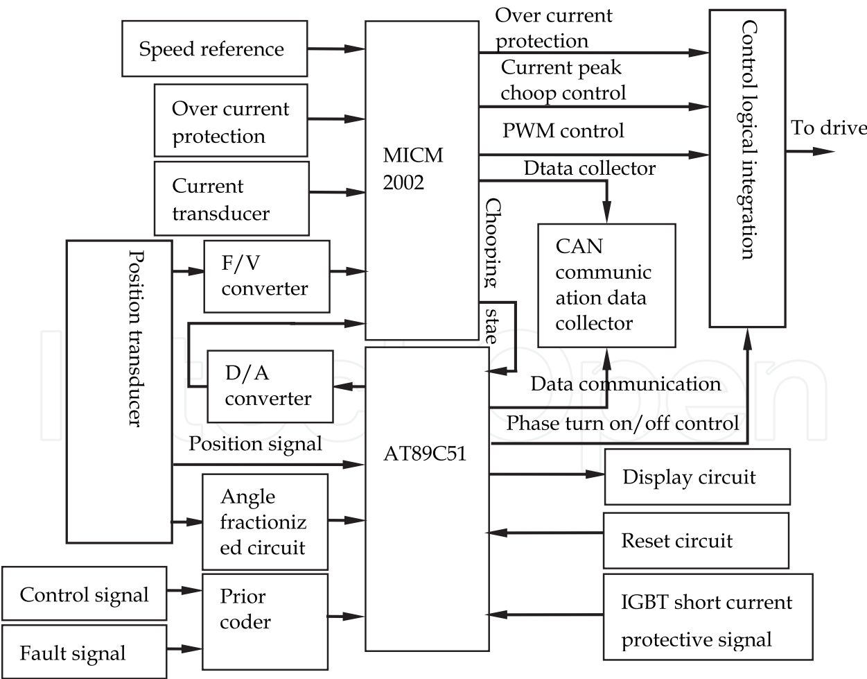
Fig. 13. Control circuit structure of SRD systems
