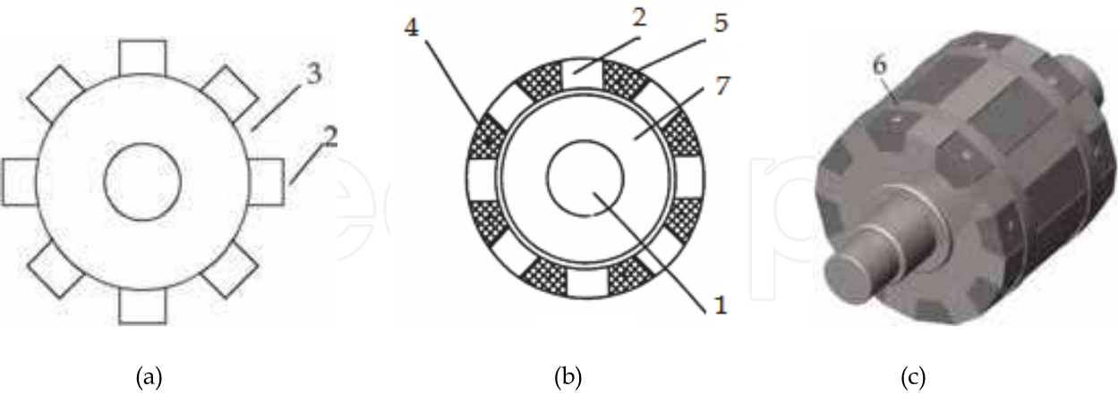
Fig. 5. A novel rotor structure for SRM
