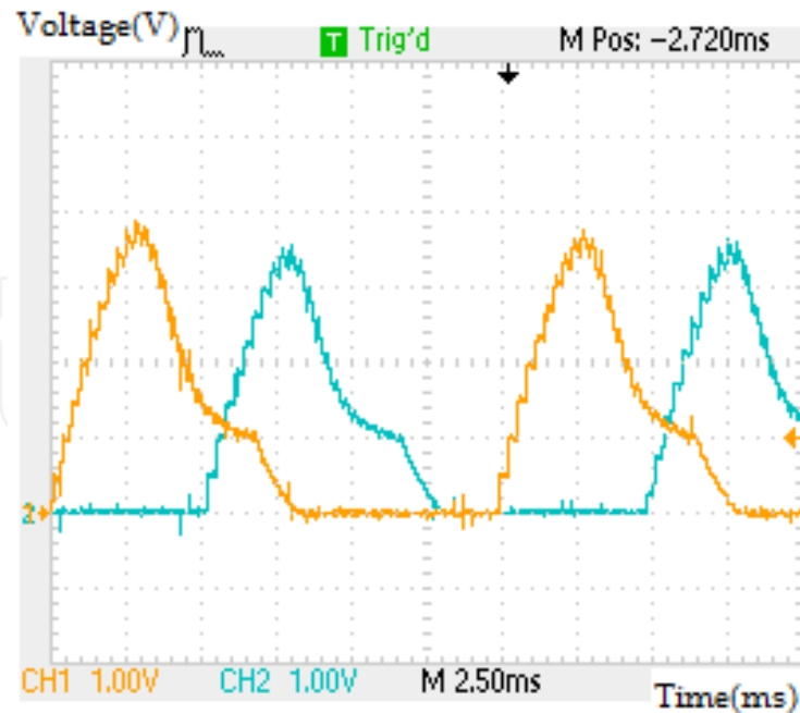
Fig. 19. Winding current waveform of n=500\text{r/min} under loaded 72Nm
