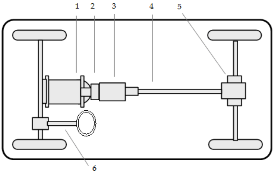
Fig. 7. Drive mode for PEUGEOT 505 SW8 conversion
