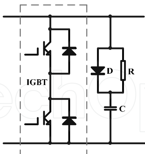
Fig. 12. IGBT snubbed electronic circuit.
