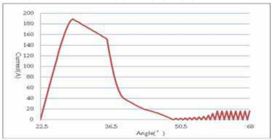
Fig. 3. Profile of designed SRM current vs. angle
