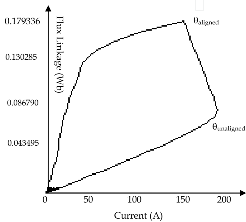
Fig. 2. Profile of designed SRM flux-linkage-current
