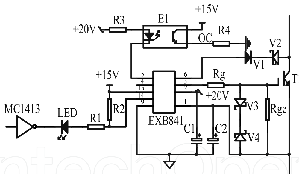
Fig. 9. IGBT drive circuit
