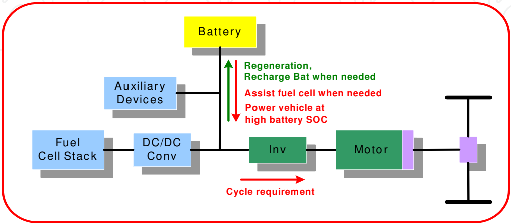
Fig. 16. Fuel Cell Hybrid Electric Vehicle configuration
