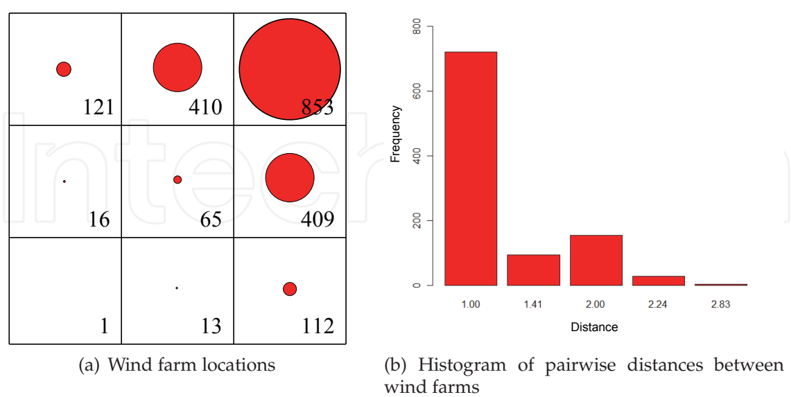
Fig. 3. Individual wind developers location results
