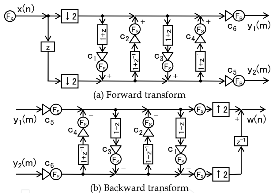
Fig. 4. The irreversible 9-7 DWT of the JPEG 2000 standard.
