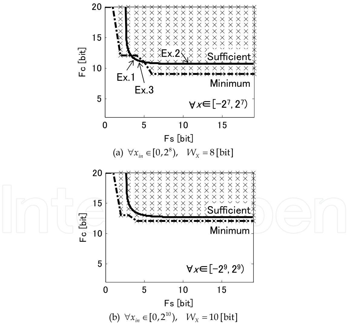
Fig. 8. Word length under the two conditions. "x" indicates (F_S, F_C) such that the DWT becomes DC lossless.
