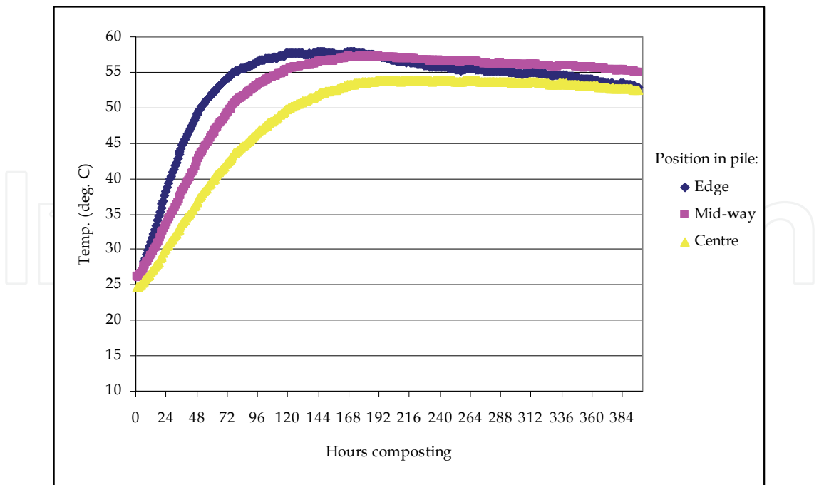
Fig. 1. Temperature development in poultry mortality composting according to position in the pile. Source: Wilkinson, unpublished.
