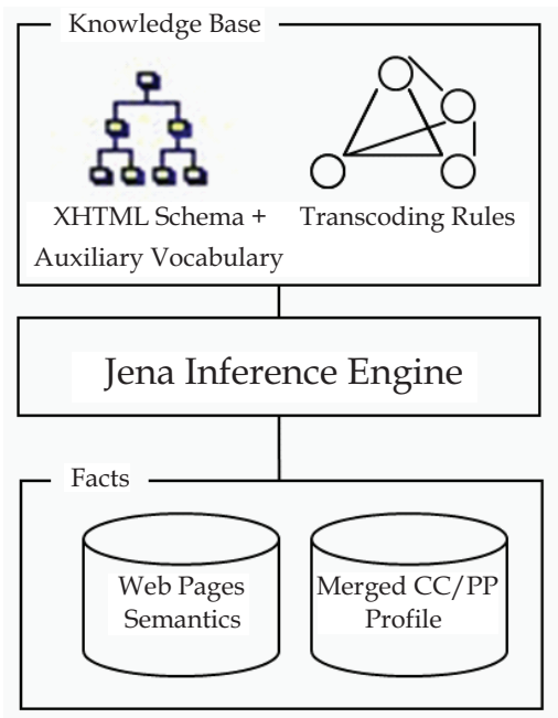
Fig. 3. Architecture of the Jena inference system
