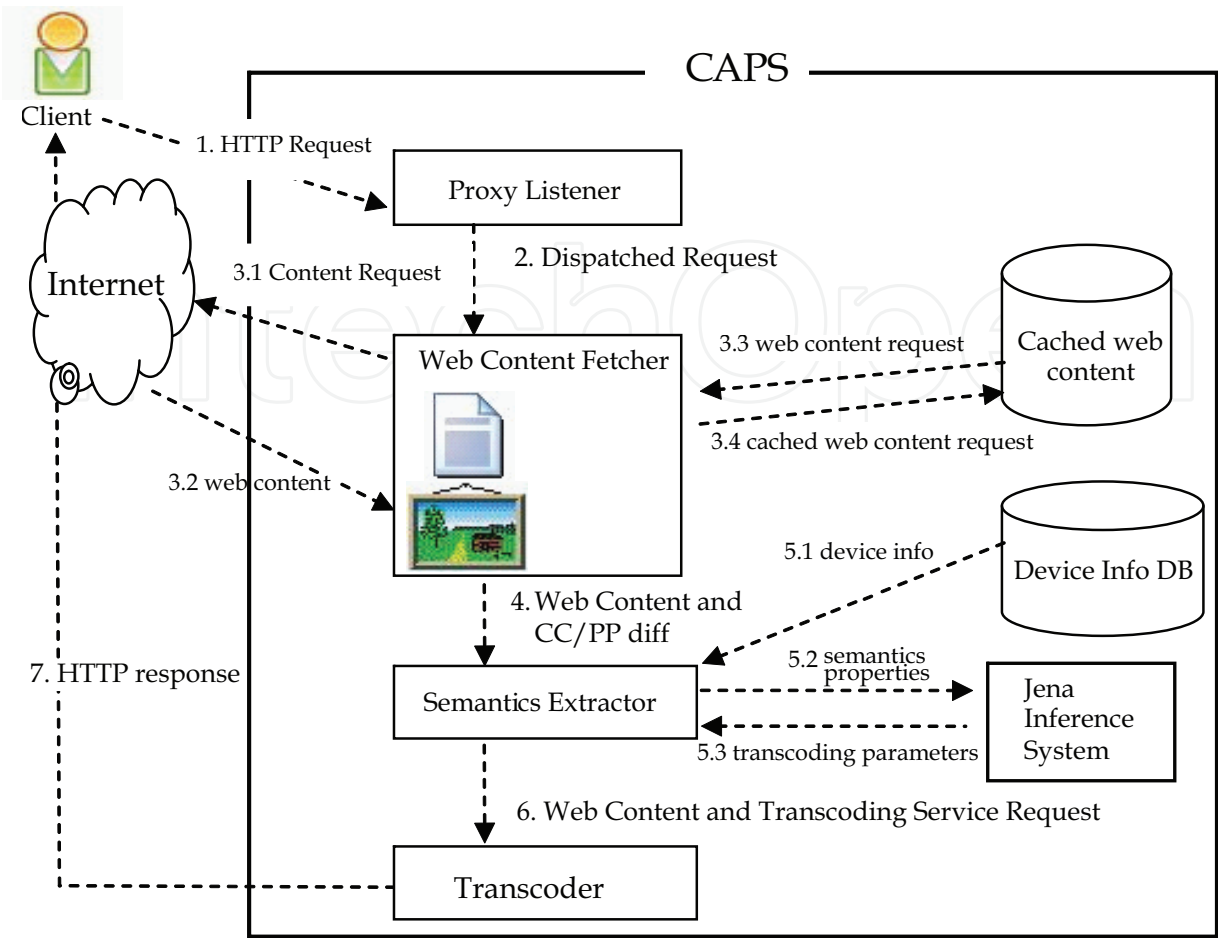
Fig. 1. System architecture of content adaptation proxy server
