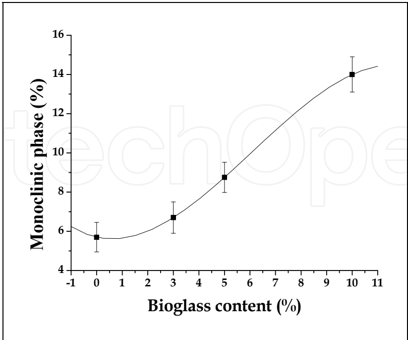
Fig. 11. Monoclinic phase concentration depending on the content of Bioglass in blocks sintered at 1300°C.
