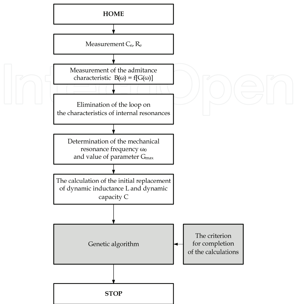
Fig. 12. Algorithm for parameter identification of dynamic model of the branch of electrical power ultrasonic transducer The initial value of the dynamic resistance R_m is calculated by selecting the characteristics shown in Fig. 9 point with coordinates (G_{max}, B_e) . In this point there is a mechanical resonance of the transducer and is a good approximation condition.
