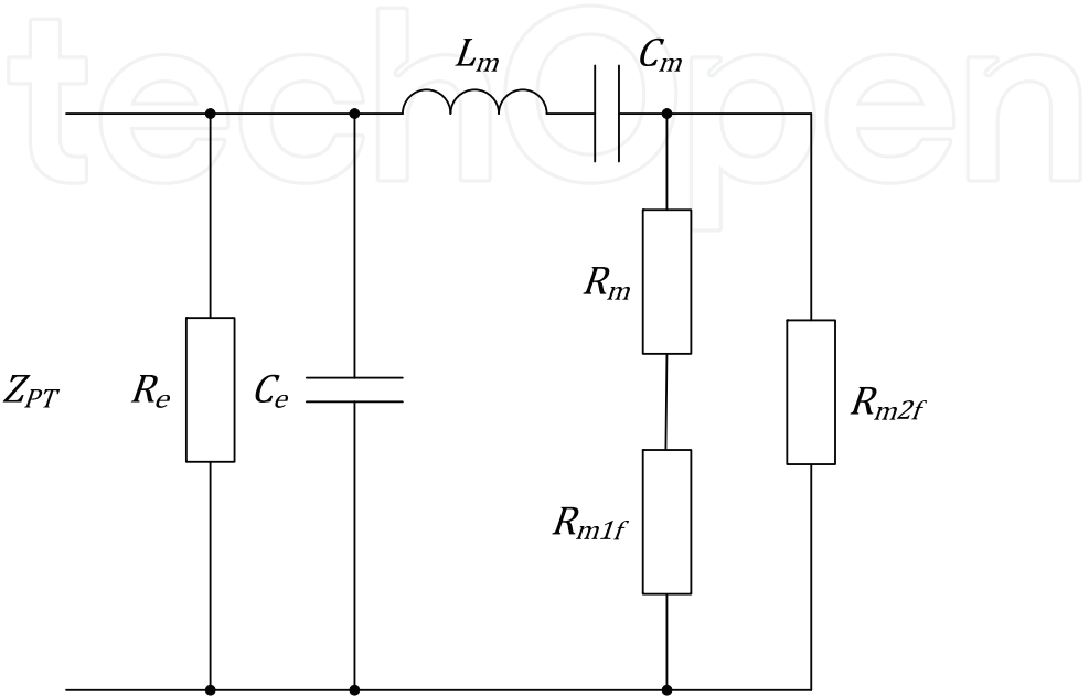
Fig. 7. Non-linear electrical model of piezoelectric ceramic transducer
