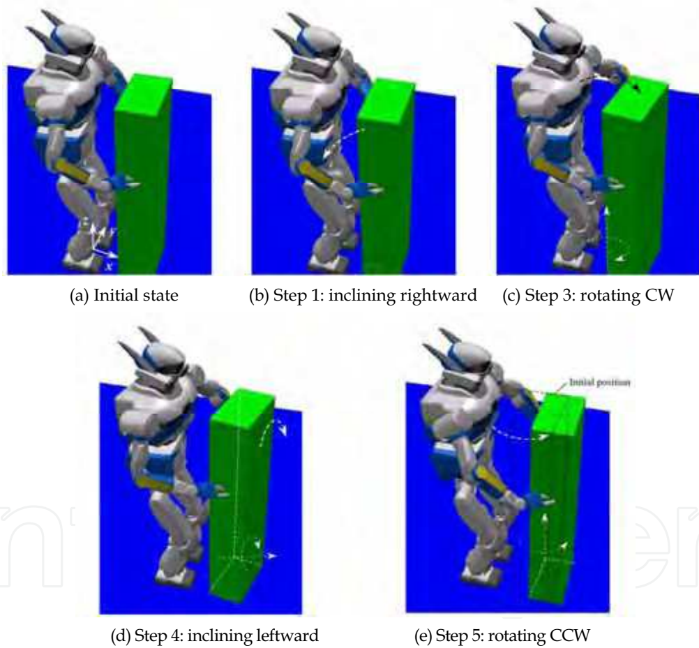
Figure 8. Simulation results of pivoting manipulation. Starting from the initial state (a), first the robot inclines the object (b) to support it on a vertex and then turns it horizontally clockwise (c). After repositioning in a horizontal position, the object is inclined on the support of another vertex (d) and turned counter-clockwise to advance the object in a parallel position with the initial one
