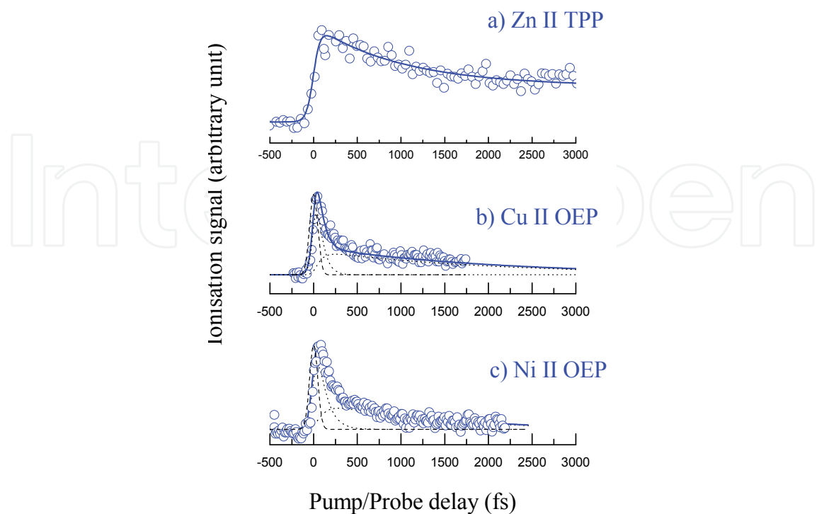
Fig. 8. Ion signals of (a) [ZnTPP] + , (b) [CuOEP] + and (c) [NiOEP] + as a function of time delay between the pump (400 nm) and the probe (800 nm)
