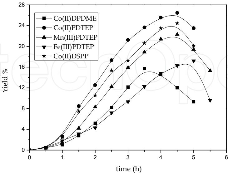
Fig. 14. Yields of cyclohexanol and cyclohexanone in the oxidation of cyclohexane catalyzed by disulphide-derivatised M(DP). Reaction conditions: cyclohexane 1000 mL, catalyst 0.02 mmol, temperature 150 °C, pressure 0.8 MPa.
