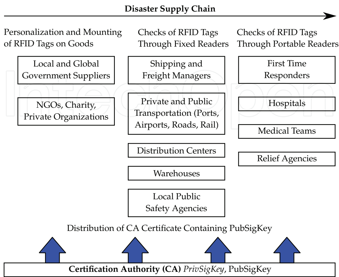
Fig. 8. Deployment workflow
