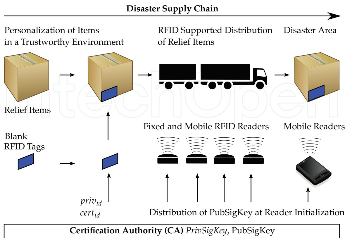
Fig. 7. Proposed system architecture for RFID secured relief item distribution
