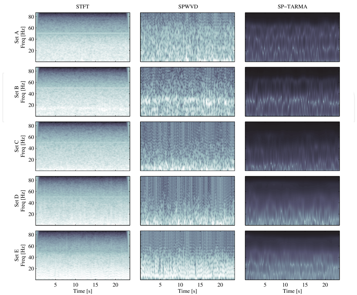
Fig. 2. Estimated TFR using the three different estimation approaches considered for exemplary signals from each class (A to E). STFT - short time Fourier transform, SPWVD - smoothed pseudo Wigner-Ville distribution, and SP-TARMA - parametric TFR based on SP-TARMA model.
