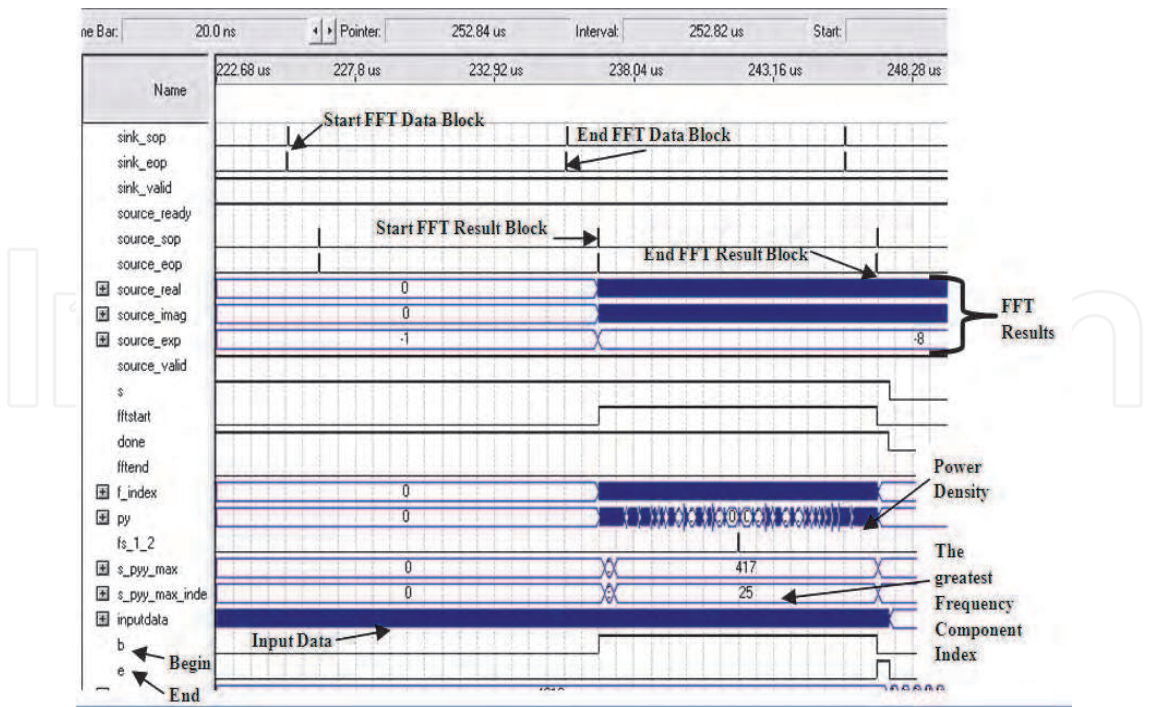
Fig. 9. FFT Simulation Results
