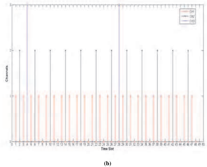
Fig. 13. Comparison between scheduling techniques(a) round-robin (cannot schedule the given signals) and (b) HMS (can optimally schedule them using the available ADC)
