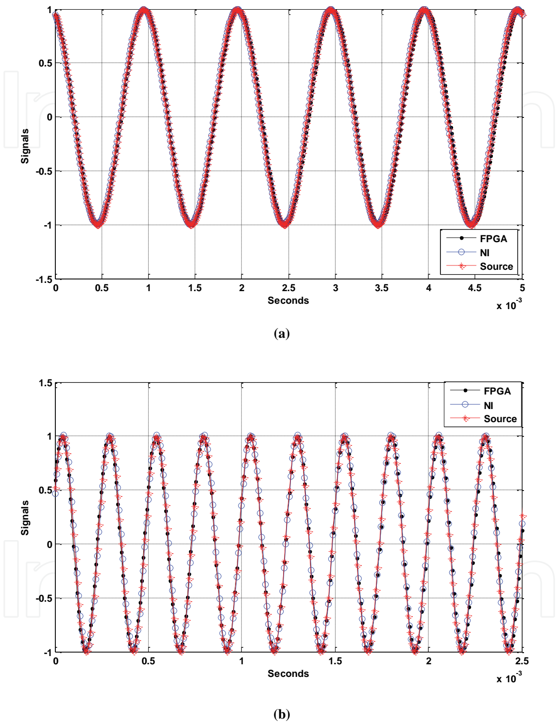
Fig. 2. Comparison between FPGA-based, NI-based DAQs (a) 1 KHz sine wave (b) 4 KHz sine wave in sequential channel DAQ
