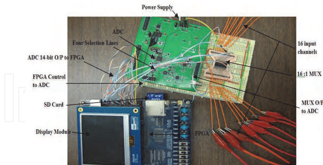
Fig. 8. FPGA Prototype of 16 multiplexed input channels ASAP
