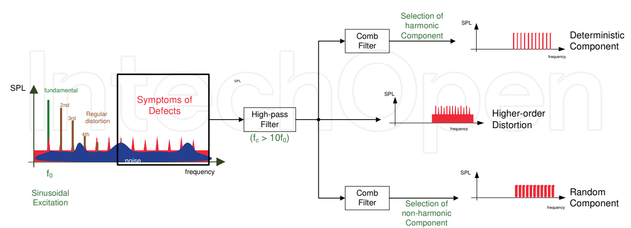
Fig. 10. Separation of the deterministic and random distortion components using a sinusoidal stimulus
