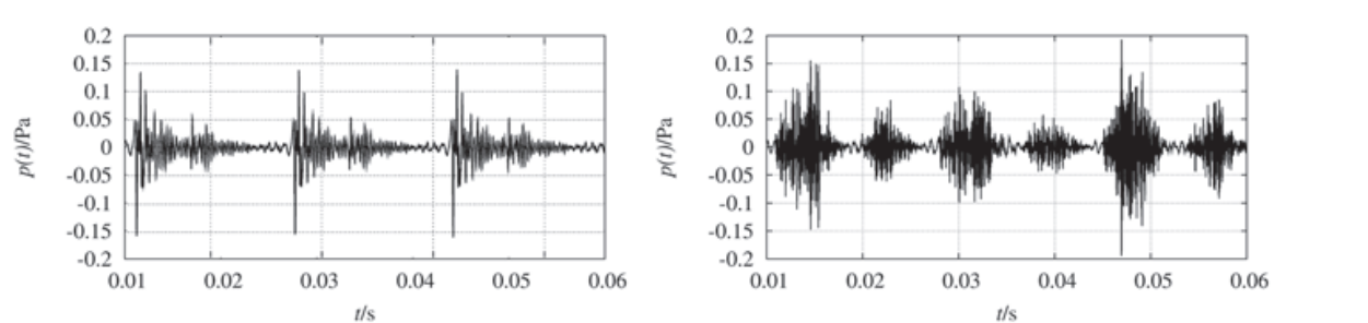
Fig. 11. Waveform of deterministic distortion component (left) caused by a buzzing loose joint and random distortion component (right) generated by an air leak
