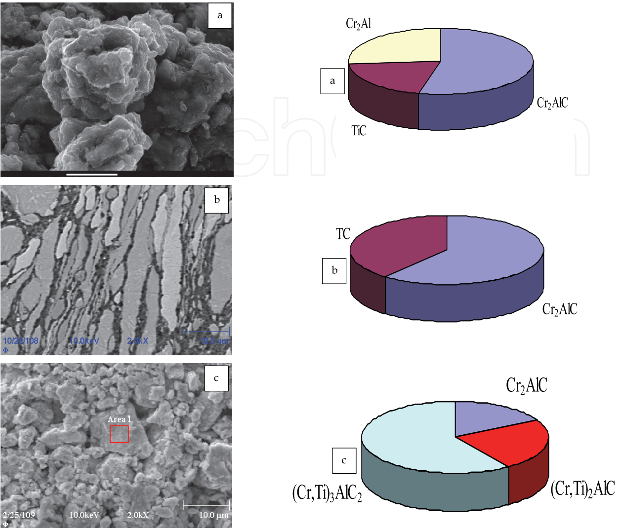
Fig. 5. Structure of the mechanically activated mixture ( x = 1.5 ) and the composition of synthesis products. MA1 (a), MA2 (b), and MA3 (c). with an average size of >10\text{ }\mu\text{m} (see Fig. 5a). The layered structure is observed for the agglomerates in the MA2 mode (see Fig. 5b). The thickness of titanium and chromium layers is from 2 to 10\text{ }\mu\text{m} that of aluminum is less than 0.5\text{--}1.0\text{ }\mu\text{m} , and that of carbon (ash) is less than 100\text{ nm} . In the MA3 mode, the mixture has a fine well-mixed structure. The average size of the agglomerates is 10\text{--}20\text{ }\mu\text{m} , and the size of particles or layers is mostly <1.0\text{ }\mu\text{m} . The amount of agglomerated particles is \sim 90\text{--}95\% of their total amount. In the first case, the main phase of the synthesized products is \text{Cr}_2\text{AlC} (54%), although the \text{TiC} (21%) and \text{Cr}_2\text{Al} (23%) are also present. In the second case, chromium aluminide is absent; the \text{Cr}_2\text{AlC} content increases to 66%, and that of \text{TiC} increases to 34%. In the MA3 mode, the sample consists of three MAX phases: (\text{Cr,Ti})_3\text{AlC}_2 , \text{Cr}_2\text{AlC} , and (\text{Cr,Ti})_2\text{AlC} . As is evident from the data of Table 4, none of considered MA modes allowed us to obtain samples completely consisting of MAX phases for the mixture with x = 0.5 . The maximal amount of the \text{Ti}_3\text{AlC}_2 phase was 55%. In addition, \text{TiC} and chromium aluminides are always present the samples. A similar situation is also observed for the mixture with x = 1 . The (\text{Cr,Ti})_3\text{AlC}_2 content does
