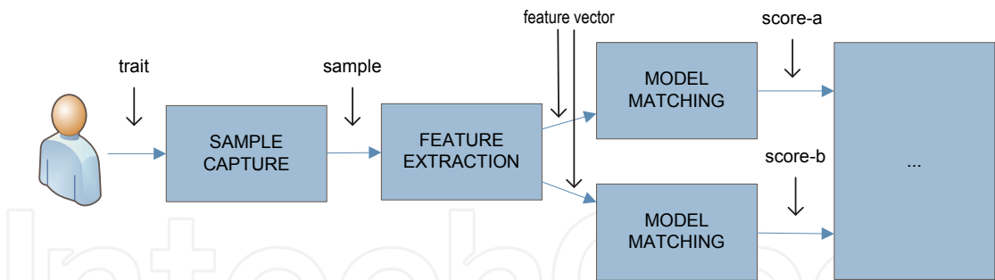
Fig. 5. Multi-matching schema.
