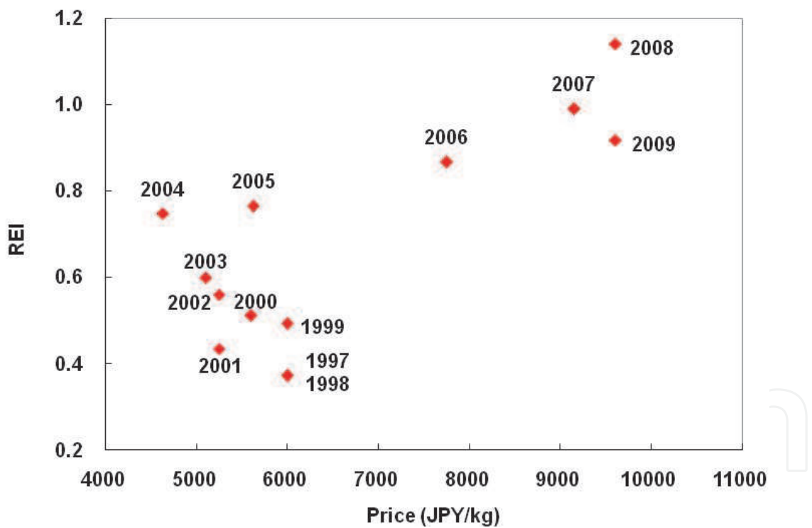
Fig. 10. Relationship between REI and pc-silicon price.
