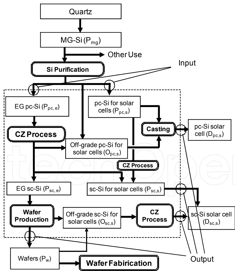
Fig. 4. Analyzed process flow of Si production.
