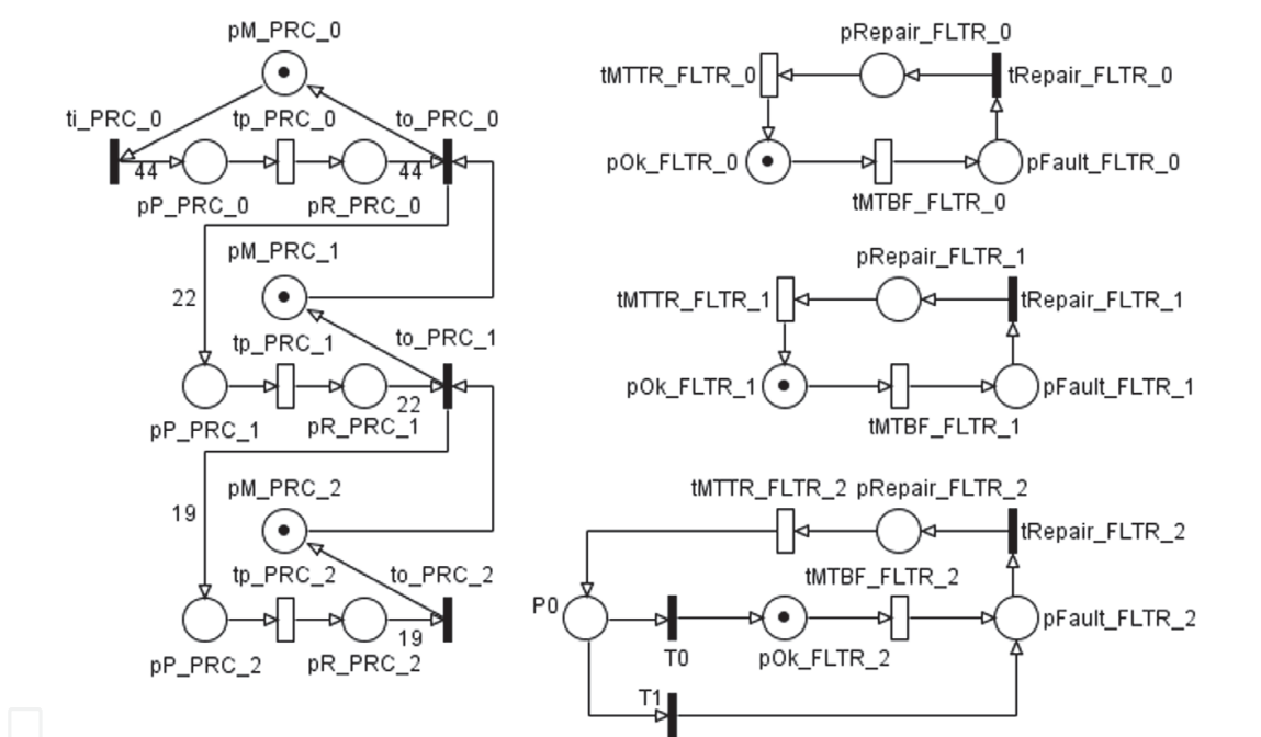
Fig. 6. Stochastic reward net for the production line.
