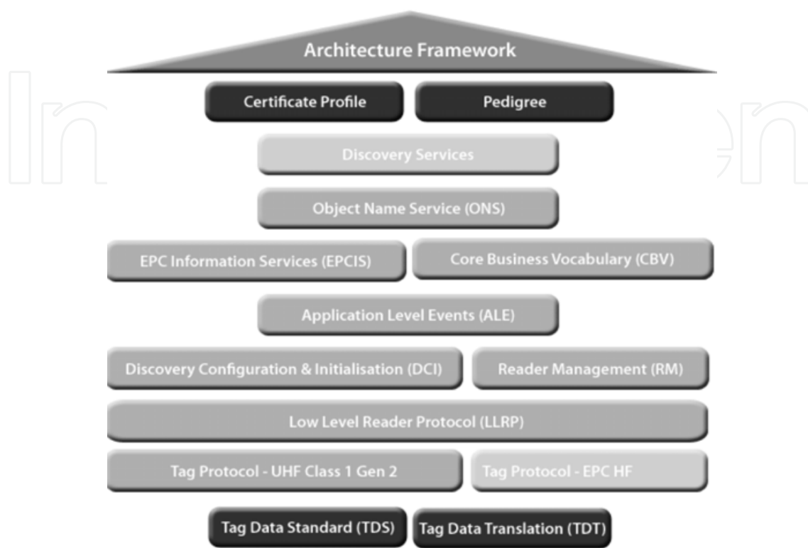
Fig. 2. EPCglobal network architecture (EPCglobal, 2005)
