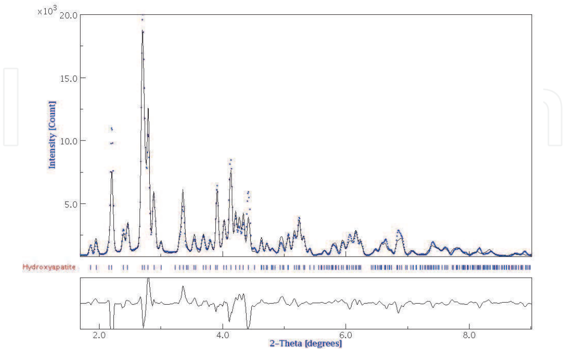
Fig. 4. Reitveld refinement of sum of all data The second step is the refinement the texture and to trace the pole figures. The all structure parameters have been and the texture of 684 diffraction patterns has been refined simultaneously by introducing the texture parameters on MAUD program.
