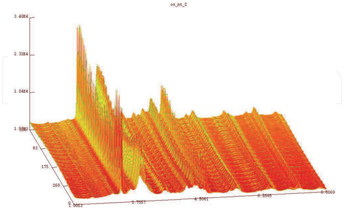
Fig. 3. 684 diffractions patterns of HAp
