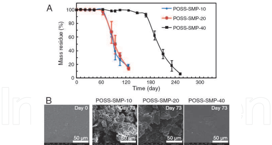
Fig. 8. In vitro hydrolytic degradation of POSS-SMPs: (A) %Mass residue of POSS-SMPs in PBS (pH 7.4) as a function of time and PLA arm length. A sample size of 3 was applied. (B) SEM micrographs of POSS-SMPs before and after 73-day incubation in PBS at 37 °C. (Adapted with permission from (Xu & Song, 2010). 2010, the National Academy of Sciences, USA.)
