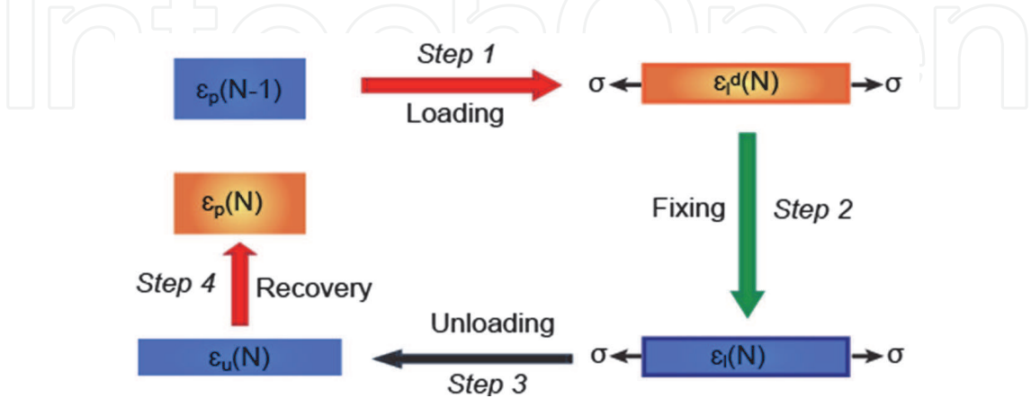
Fig. 1. Programming steps in a stress-controlled cyclic thermo-mechanical test of an SMP. Denotations: p = permanent, l = with loading, d = deformation temperature T_d , u = unloading
