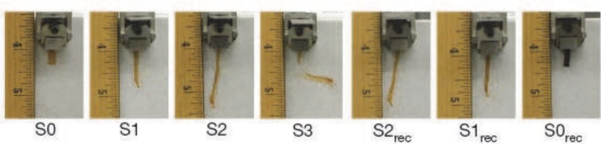
Fig. 5. Quadruple-shape memory properties of PFSA. S0: permanent shape; S1: first temporary shape ( T_d^1 : 140 °C); S2: second temporary shape ( T_d^2 : 107 °C); S3: third temporary shape ( T_d^3 : 68°C); S2 rec : recovered second temporary shape ( T_r^1 : 68°C); S1 rec : recovered first temporary shape ( T_r^2 : 107 °C); S0 rec : recovered permanent shape ( T_r^3 : 140 °C). (Adapted with permission from (Xie, 2010). 2010. Nature Publishing Group Inc.)
