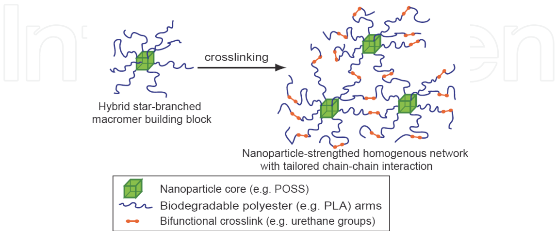
Fig. 6. Depiction of a multi-functional SMP network. (Adapted with permission from (Xu & Song, 2010). 2010, the National Academy of Sciences, USA.)
