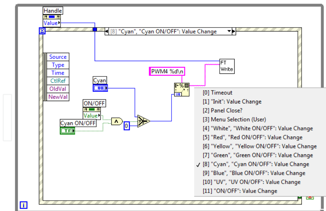
Fig. 14. Example of handling the user interface activities by event structure.
