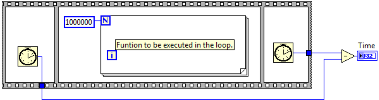
Fig. 4. Experiment of measuring execution time of one loop iteration
