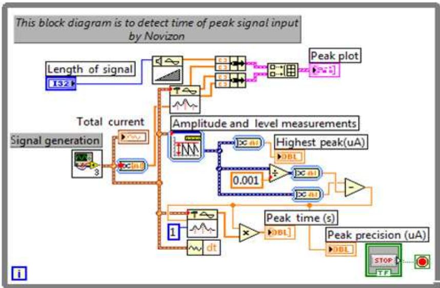
Fig. 19. LabVIEW diagram of peak detector
