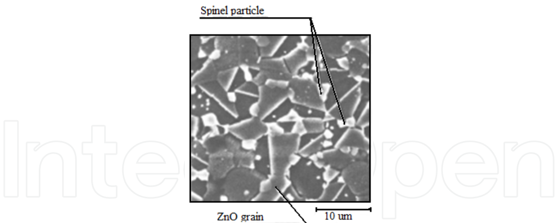
Fig. 3. Secondary-electron image of the ZnO element (Kobayashi, 1986).
