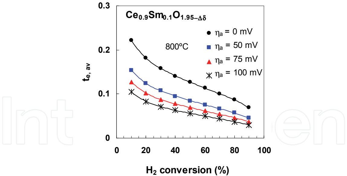
Fig. 18. Electronic transport number averaged across the membrane as function of hydrogen conversion for several values of anodic overpotential.
