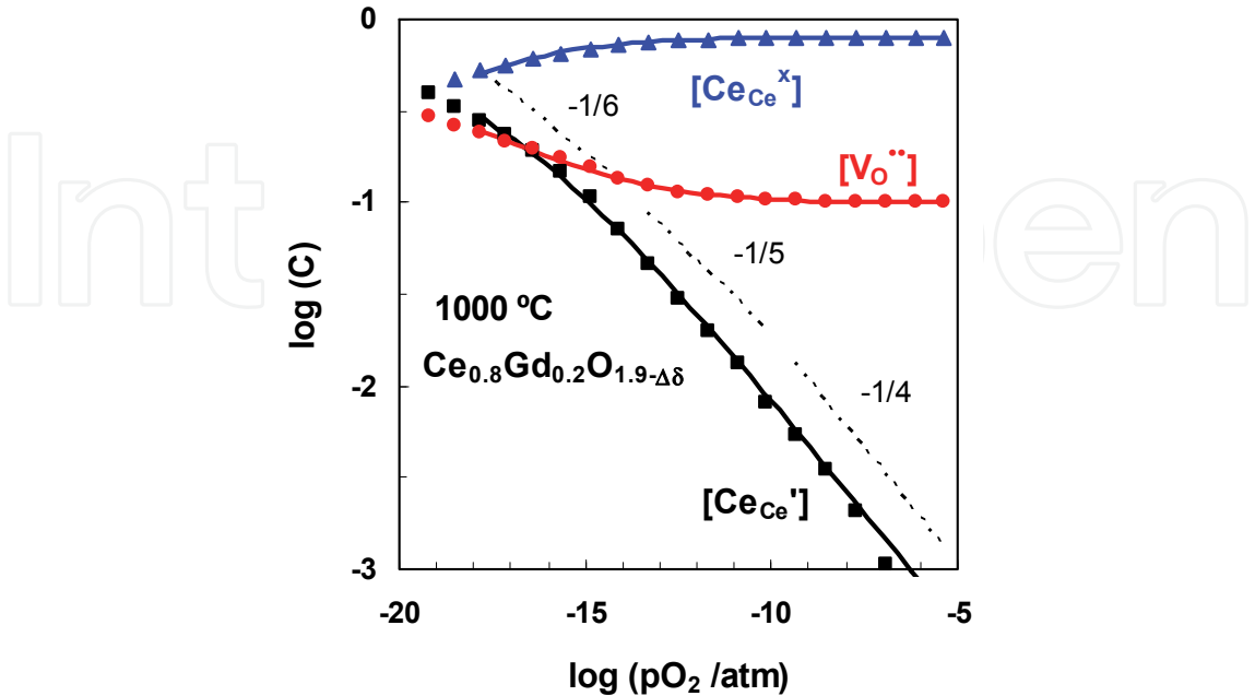
Fig. 6. Defect chemistry concentrations (molar fractions) as functions of oxygen partial pressure for \text{Ce}_{0.8}\text{Gd}_{0.2}\text{O}_{1.9-\Delta\delta} at 1000 °C. Single points correspond to the experimental values obtained from coulometric titration, whereas straight lines correspond to theoretical values using the simple defect chemistry model.
