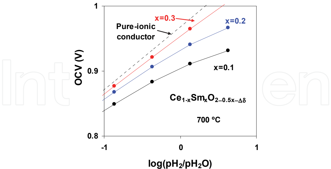
Fig. 17. Predictions of open cell voltage vs hydrogen:steam ratio for several contents of Sm in Ce_{1-x}Sm_xO_{2-0.5x-\Delta\delta} at 700 °C, based on the experimental dependence of electronic transport properties.
